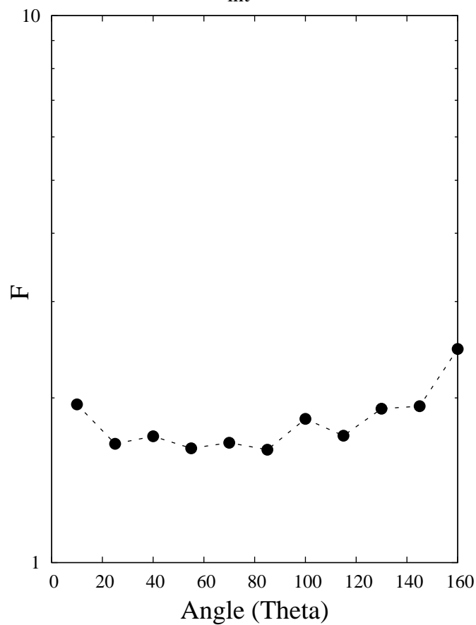
F factor - (Full energy range, MeV)
