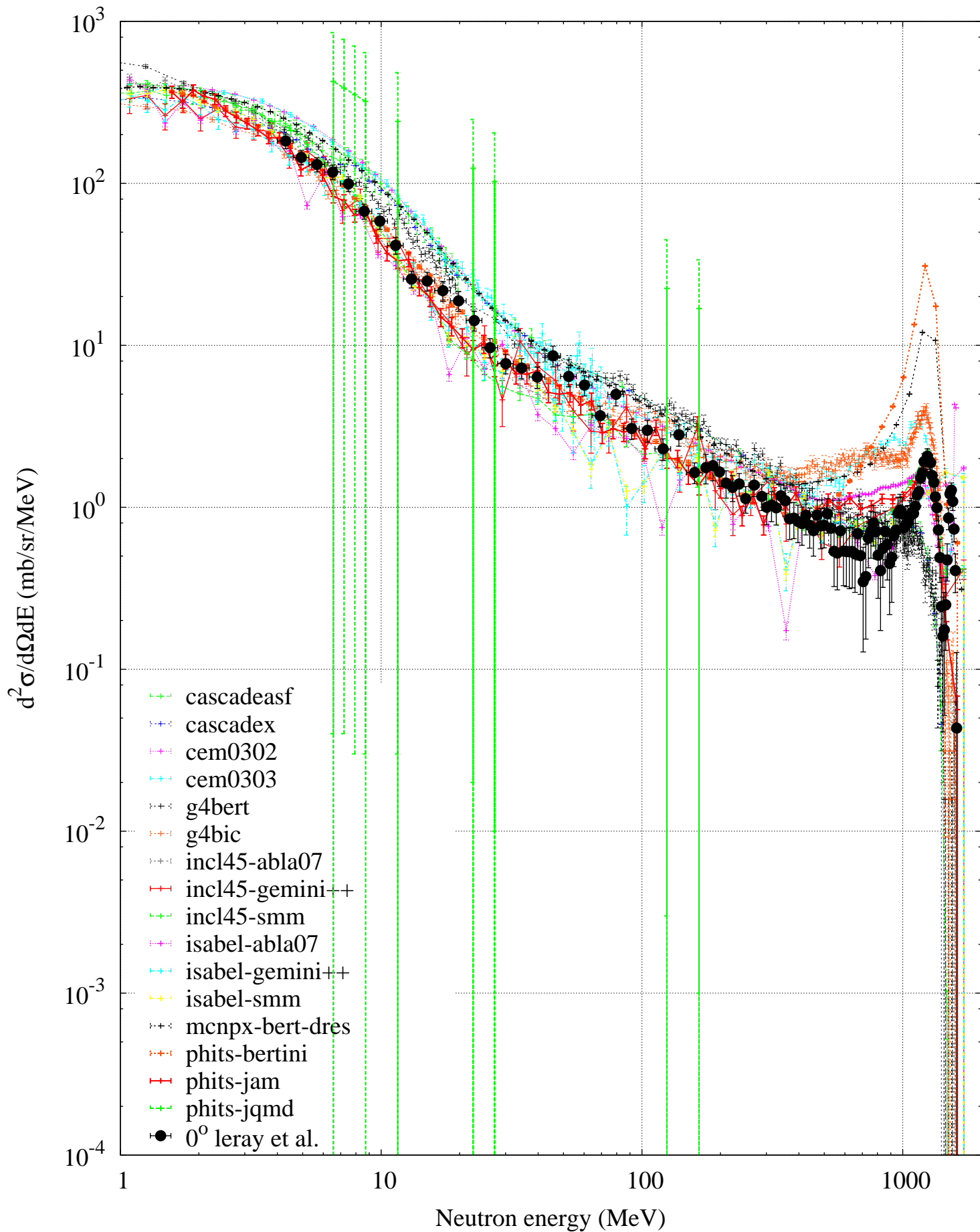
p (1600 MeV) + Pb -- Neutron spectrum
