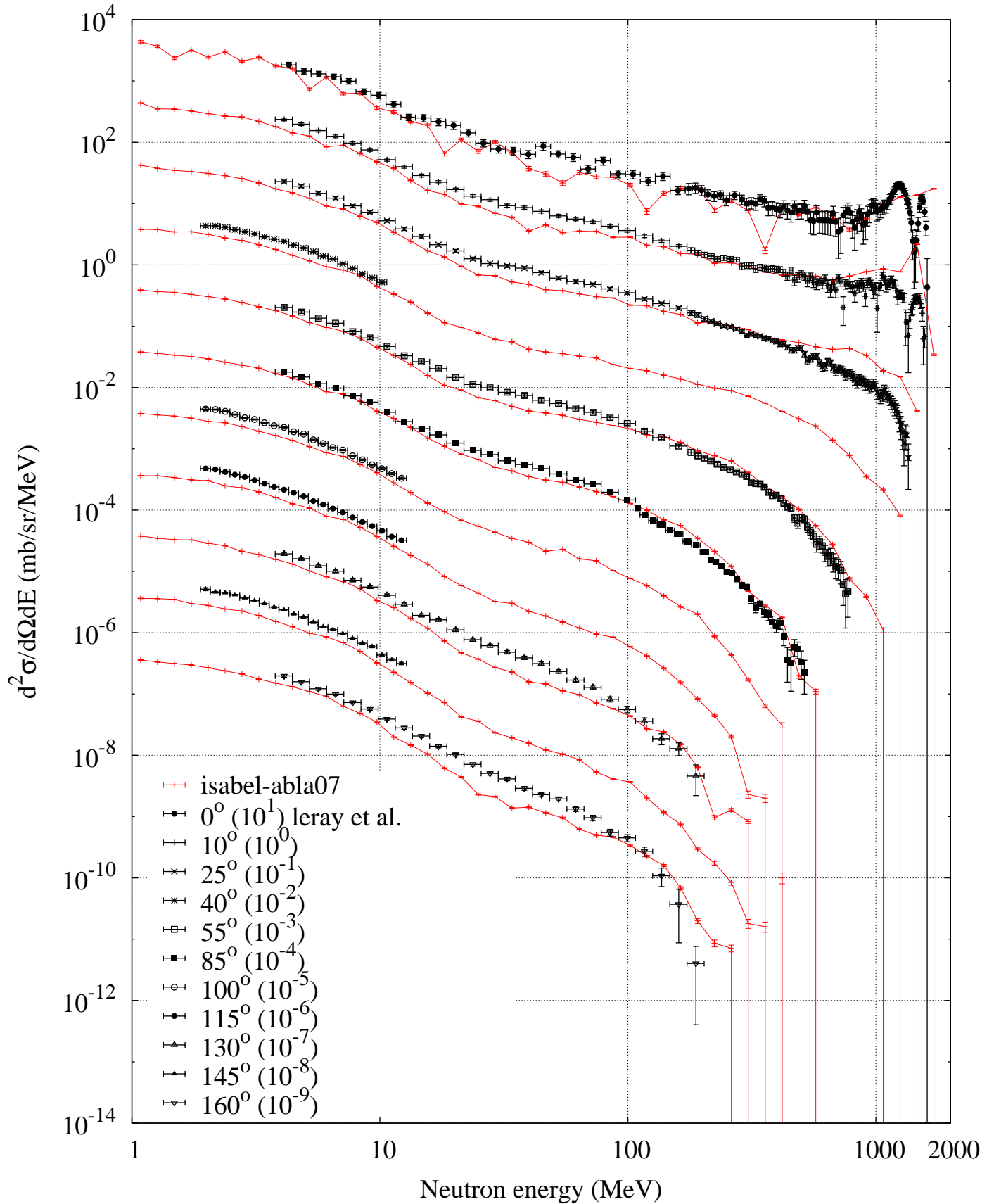
p (1600 MeV) + Pb -- Neutron spectrum
