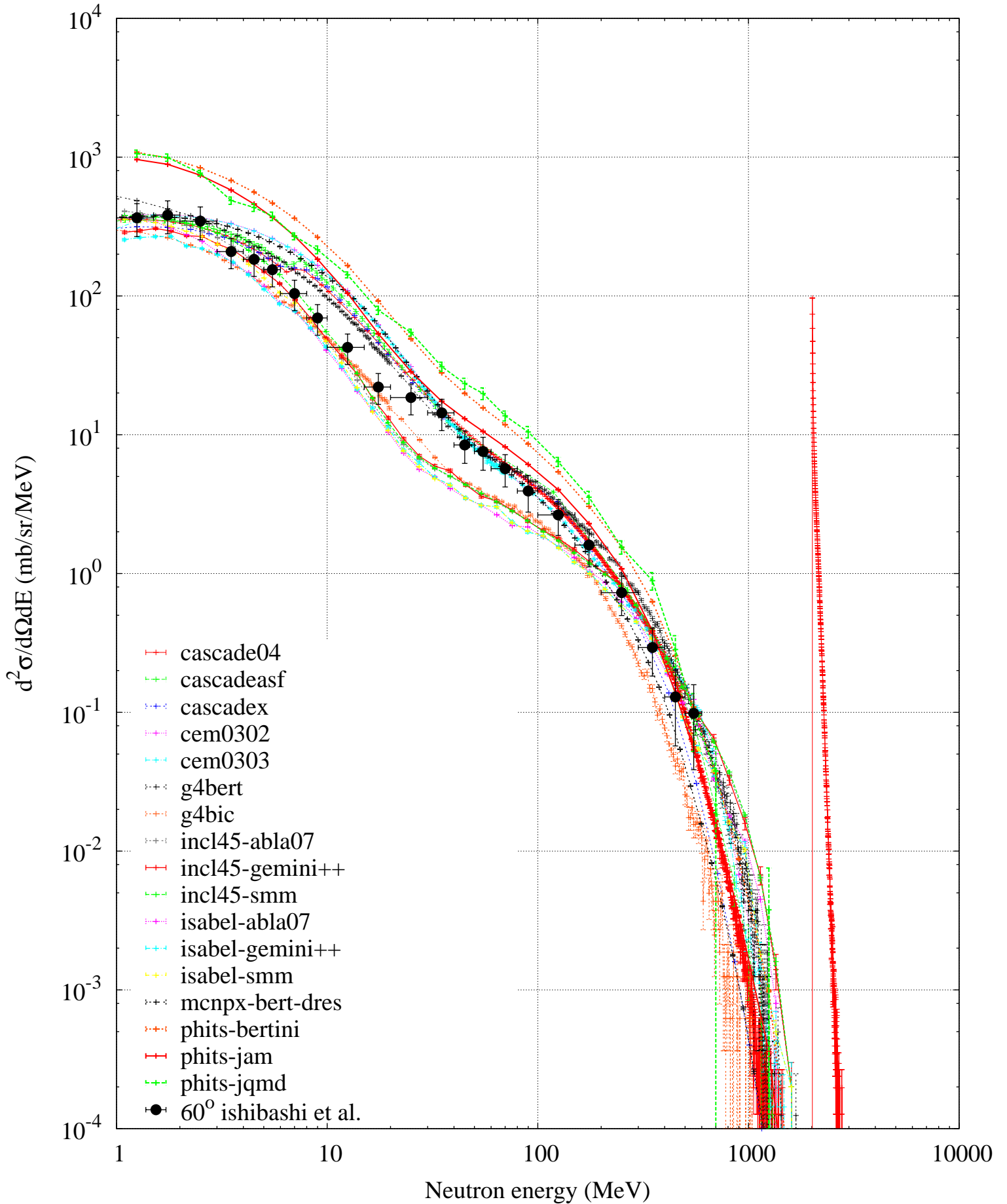
p (3000 MeV) + Pb -- Neutron spectrum
