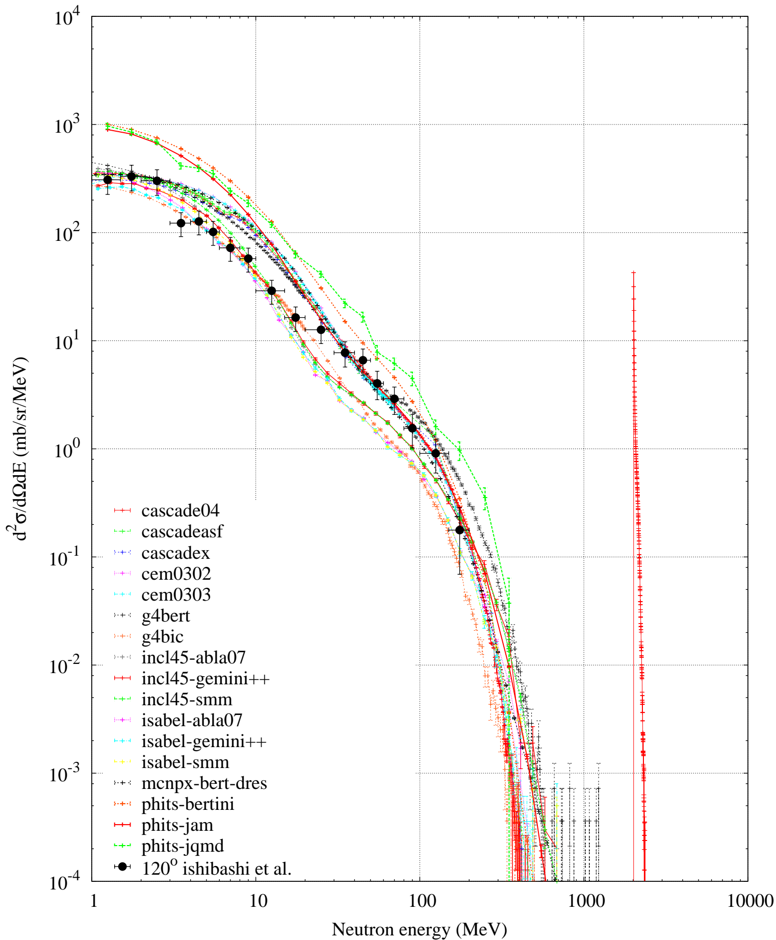
p (3000 MeV) + Pb -- Neutron spectrum
