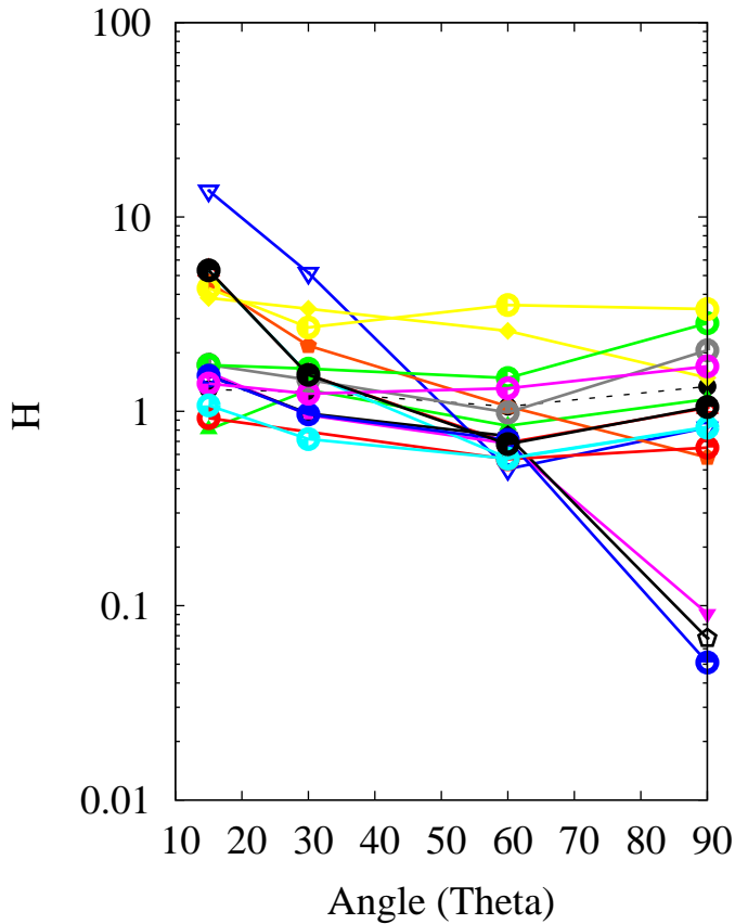
H factor - E_{\text{high}} (150+ MeV)
