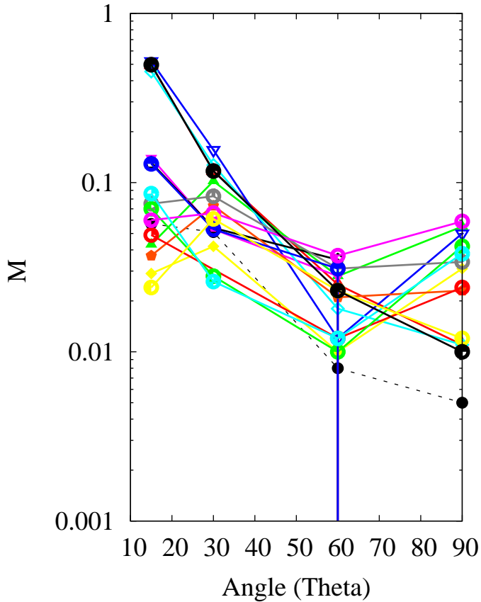
M factor - E_{\text{high}} (150+ MeV)
