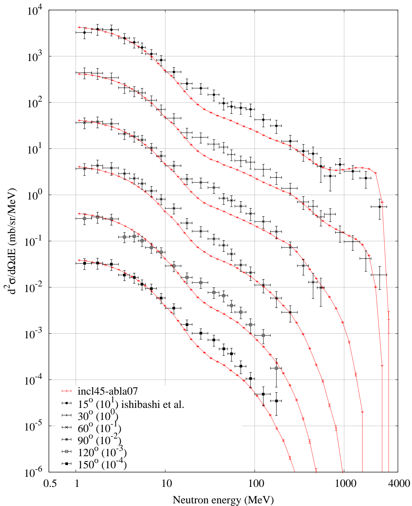
p (3000 MeV) + Pb -- Neutron spectrum
