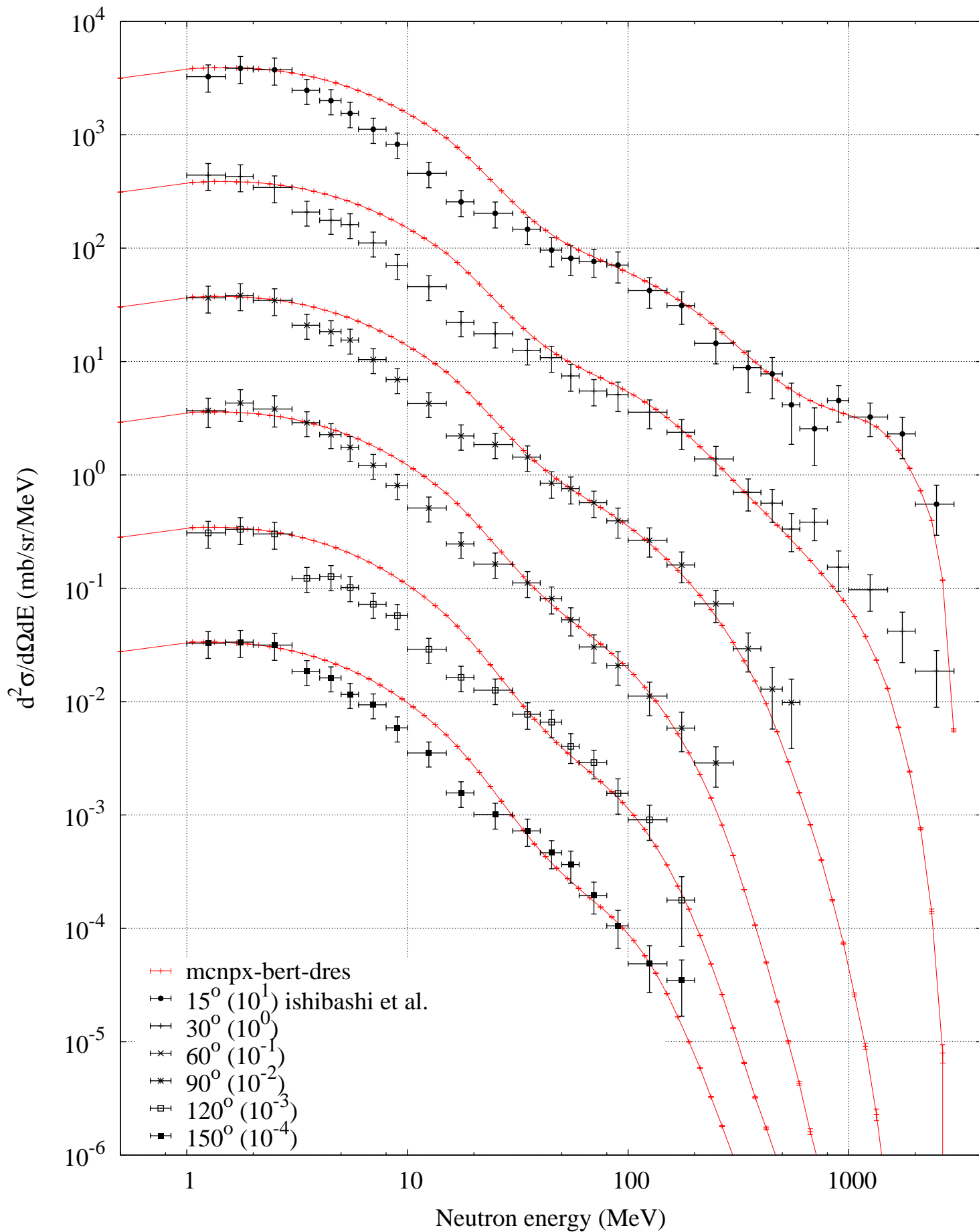
p (3000 MeV) + Pb -- Neutron spectrum
