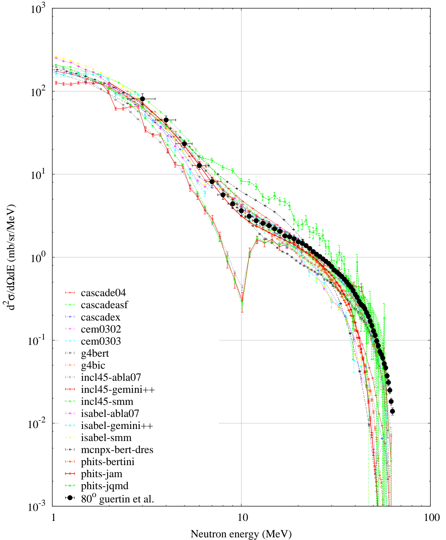
p (63 MeV) + Pb208 -- Neutron spectrum
