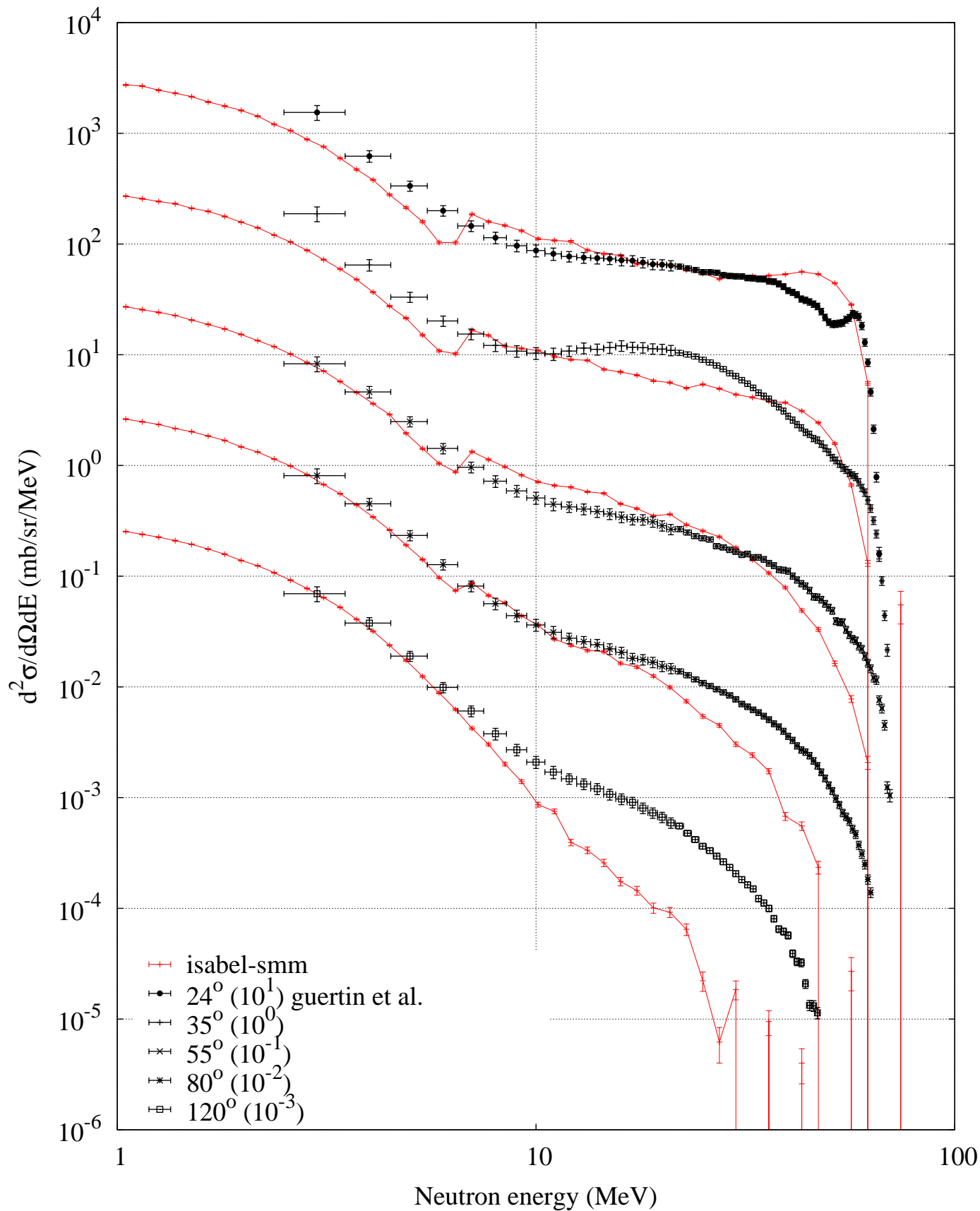
p (63 MeV) + Pb208 -- Neutron spectrum
