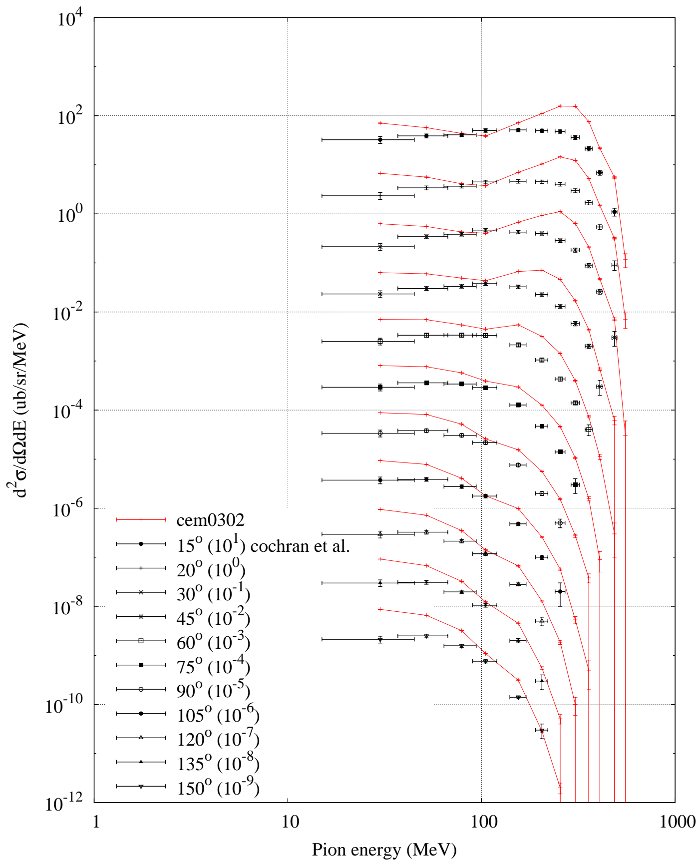
p (730 MeV) + C -- Pion minus spectrum
