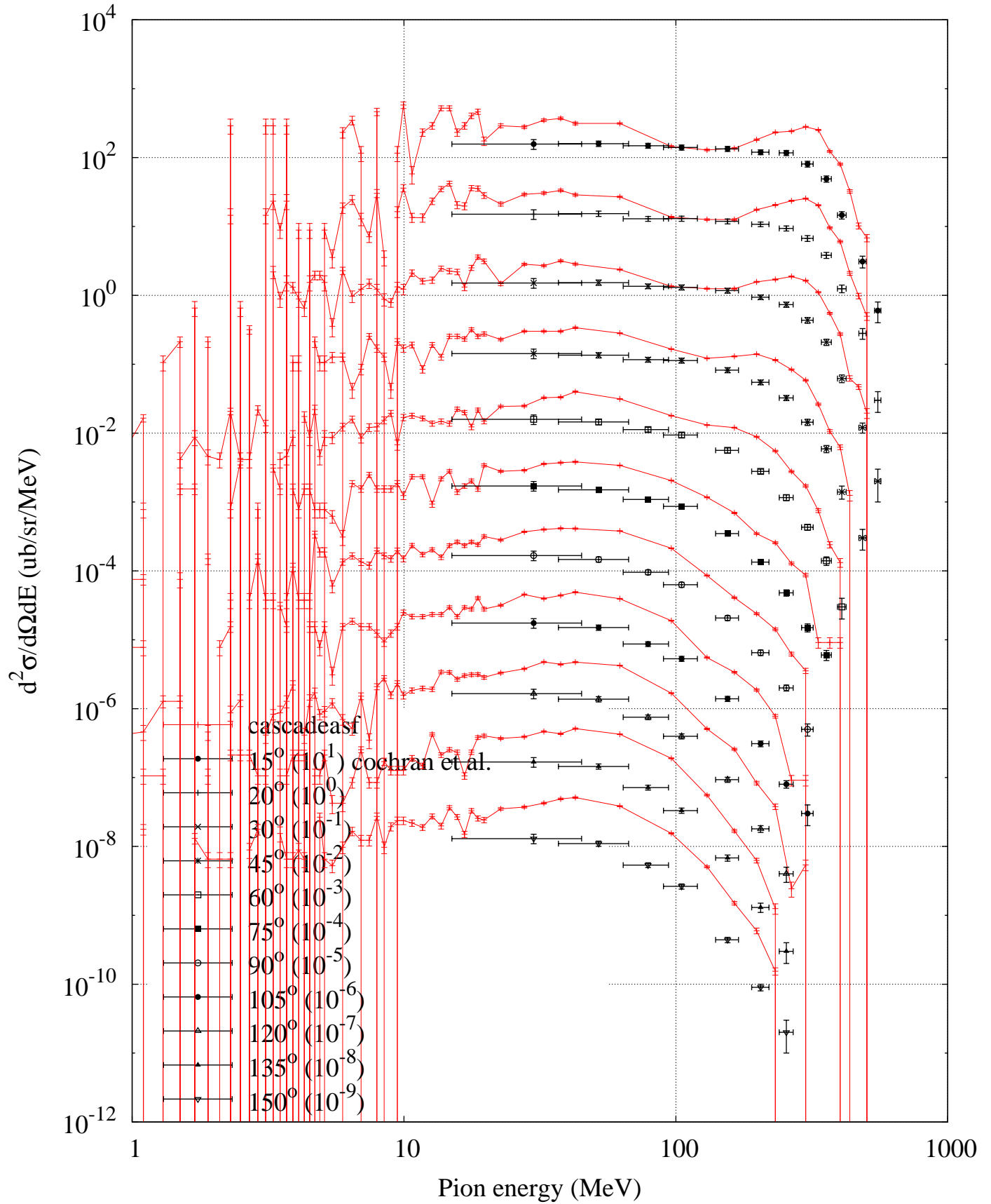
p (730 MeV) + Cu -- Pion minus spectrum
