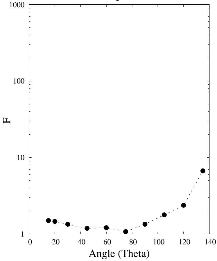
F factor - E_{\text{high}} (150+ MeV)
