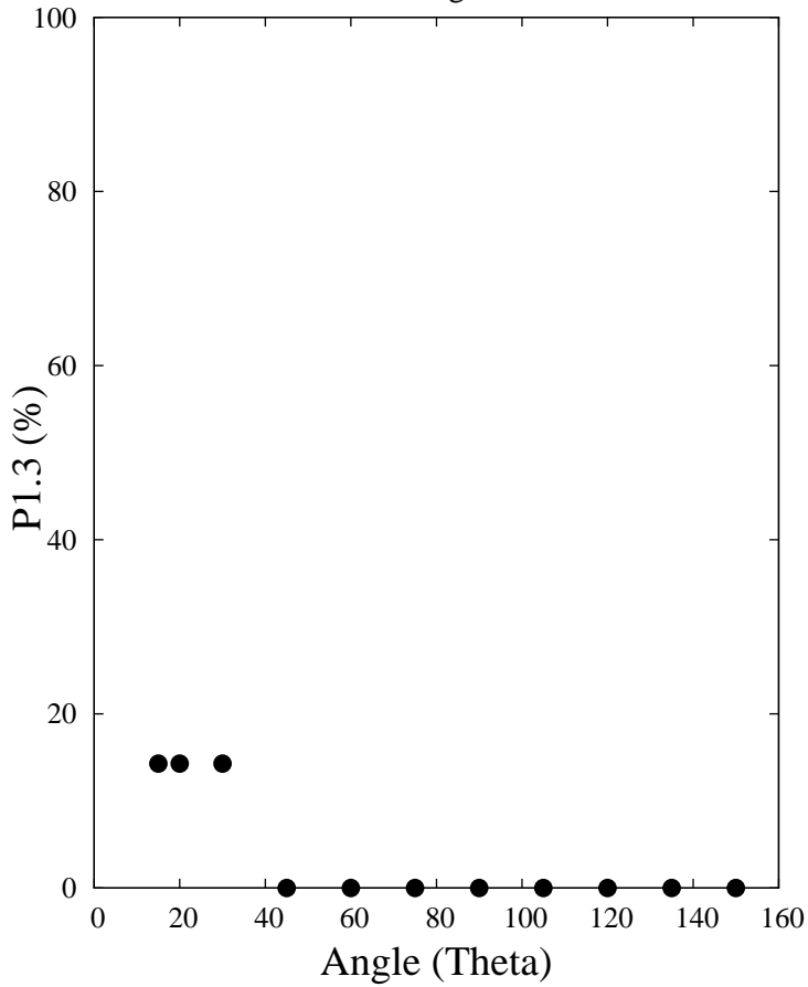
P1.3 factor - E_{high}(150+ \text{ MeV})
