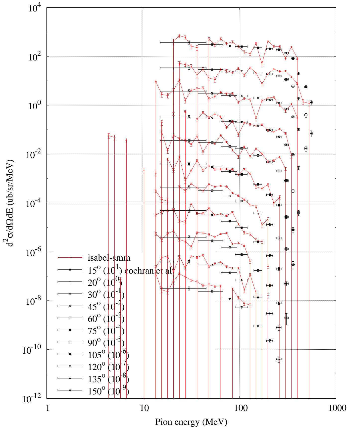
p (730 MeV) + Pb -- Pion minus spectrum
