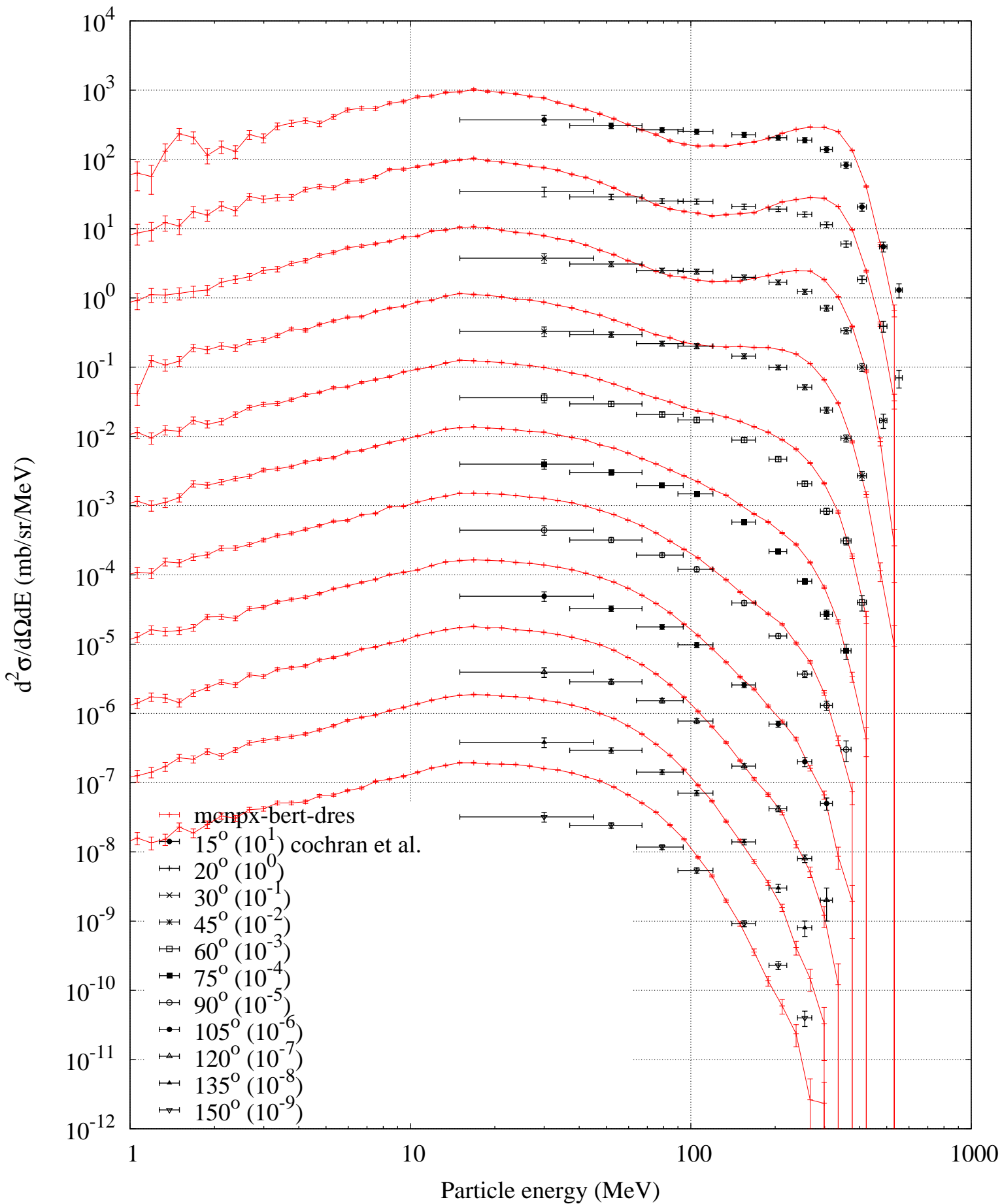
p (730 MeV) + Pb -- Pion minus spectrum
