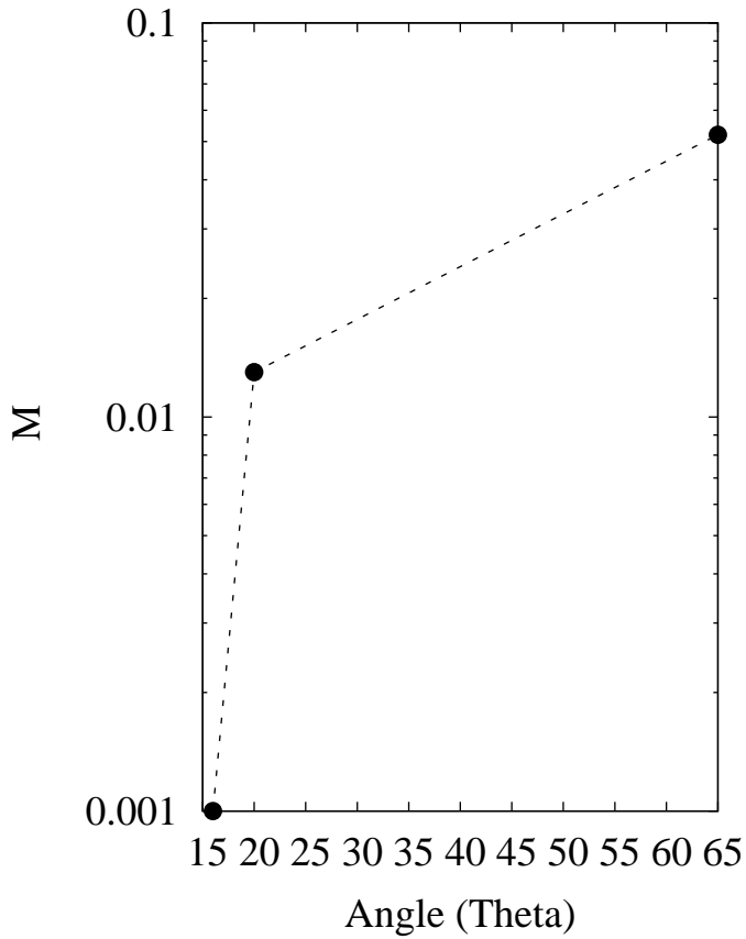
M factor - E_{\text{high}} (150+ MeV)
