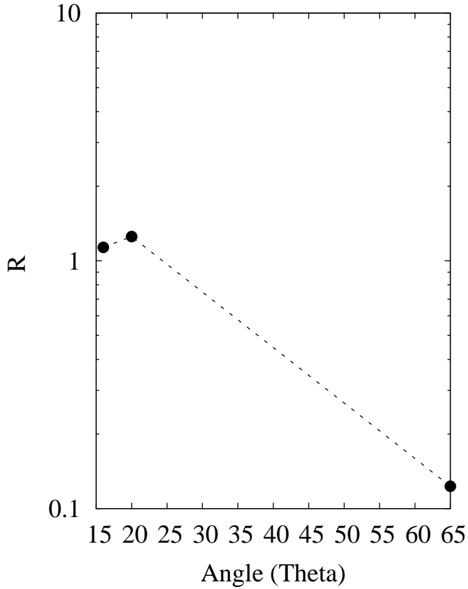
R factor - E_{\text{high}} (150+ MeV)
