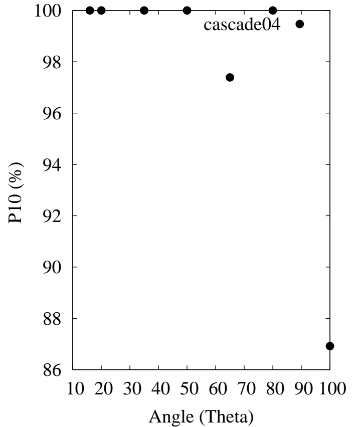
P10 factor - E_{\text{tot}} (full energy range, MeV)
