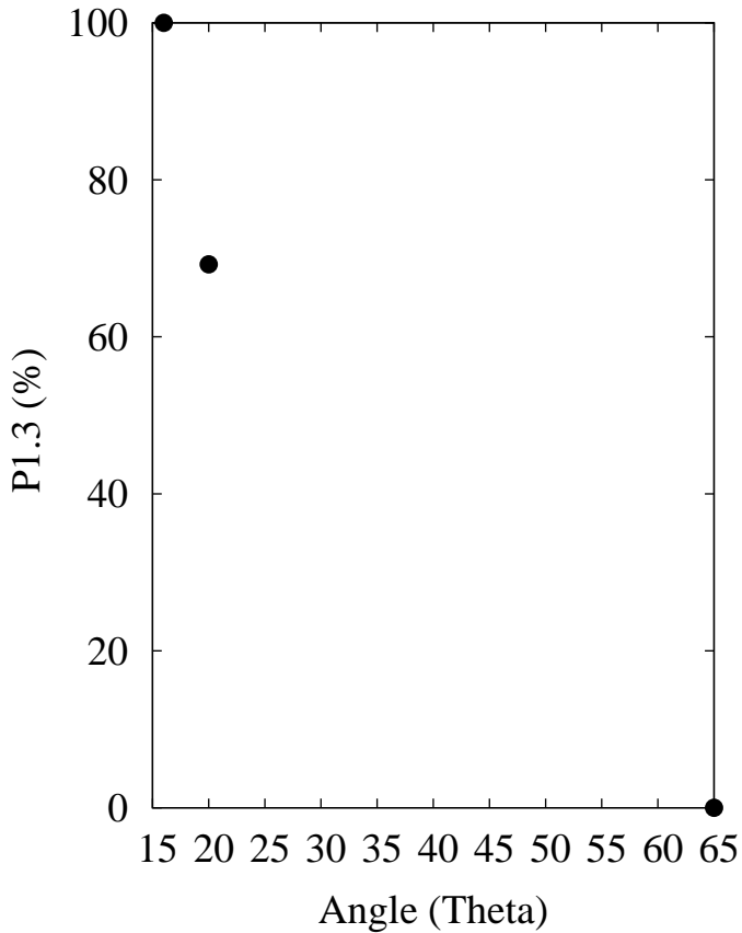
P1.3 factor - E_{\text{high}} (150+ MeV)
