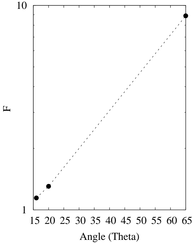
F factor - E_{\text{high}} (150+ MeV)
