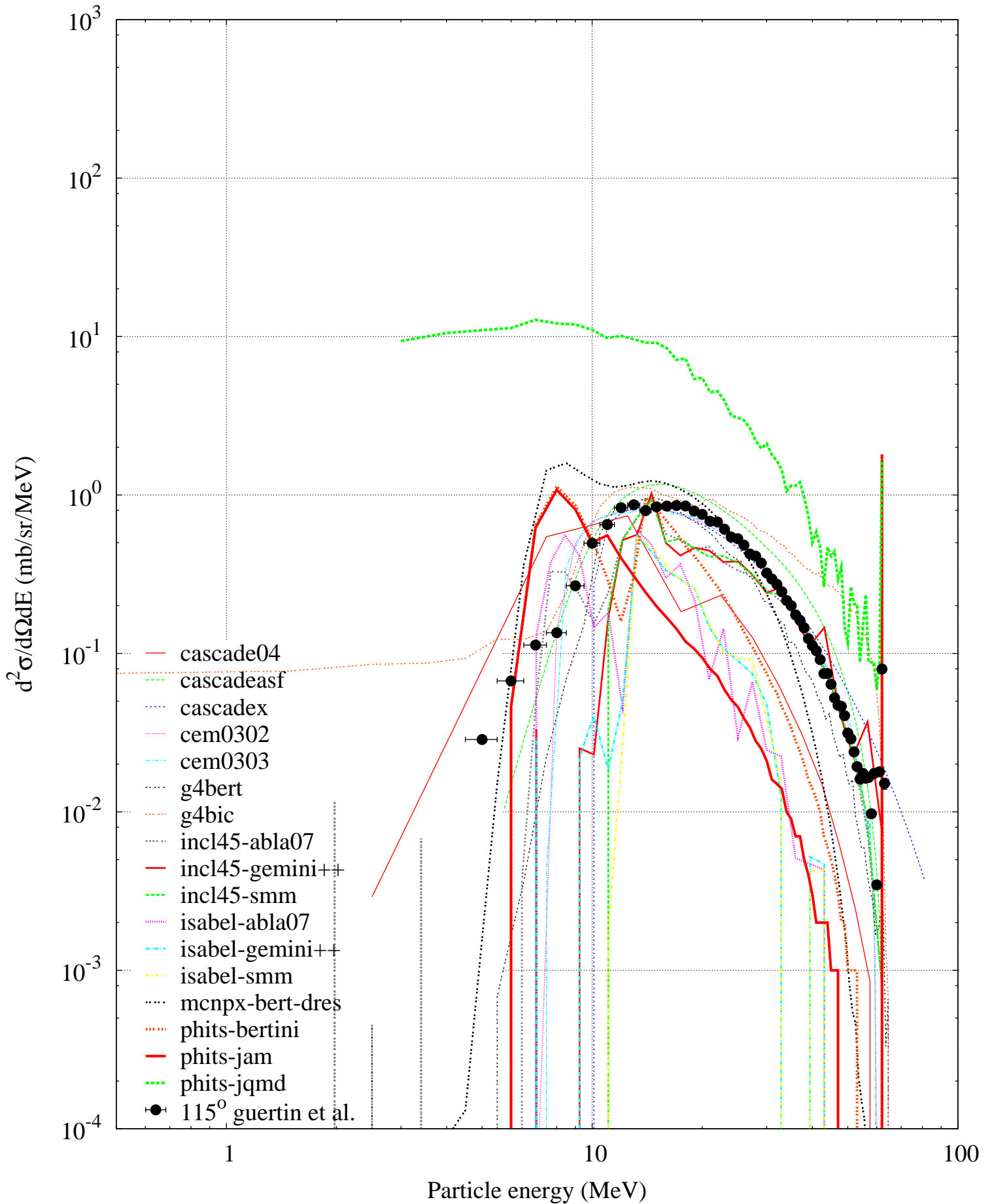
p (63 MeV) + Pb208 -- Proton spectrum
