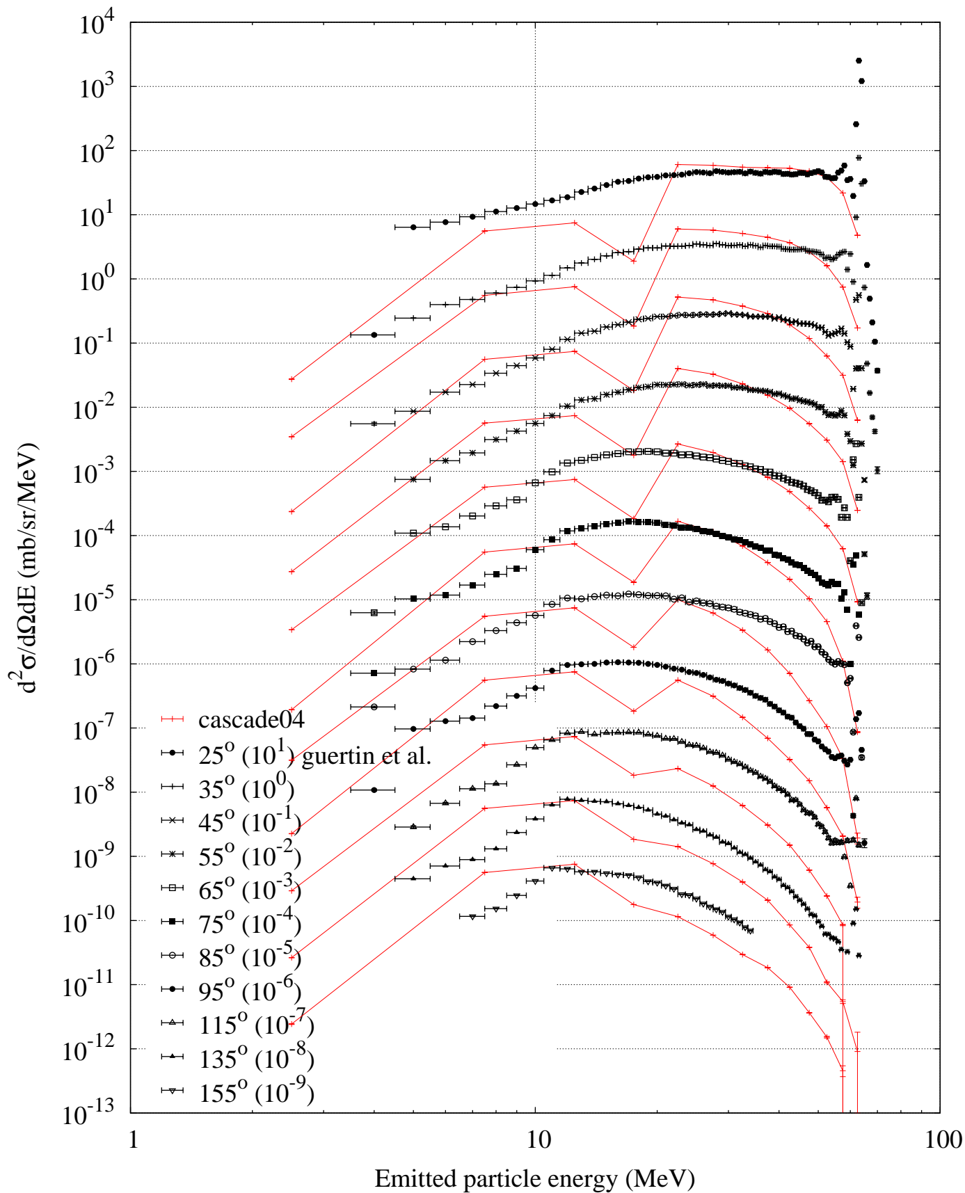
p (63 MeV) + Pb208 -- Proton spectrum
