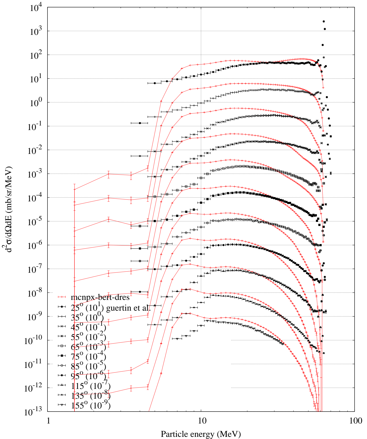
p (63 MeV) + Pb208 -- Proton spectrum
