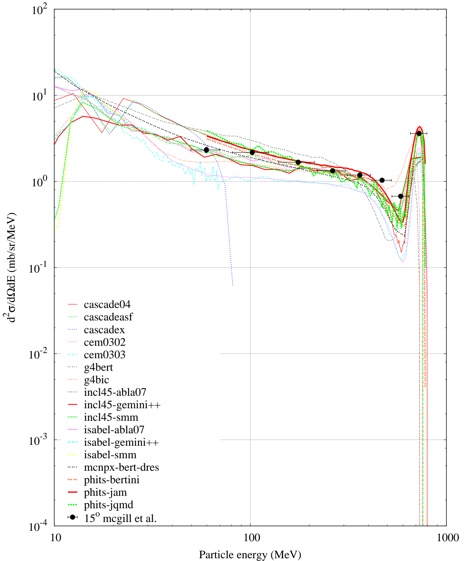
p (800 MeV) + Pb208 -- Proton spectrum
