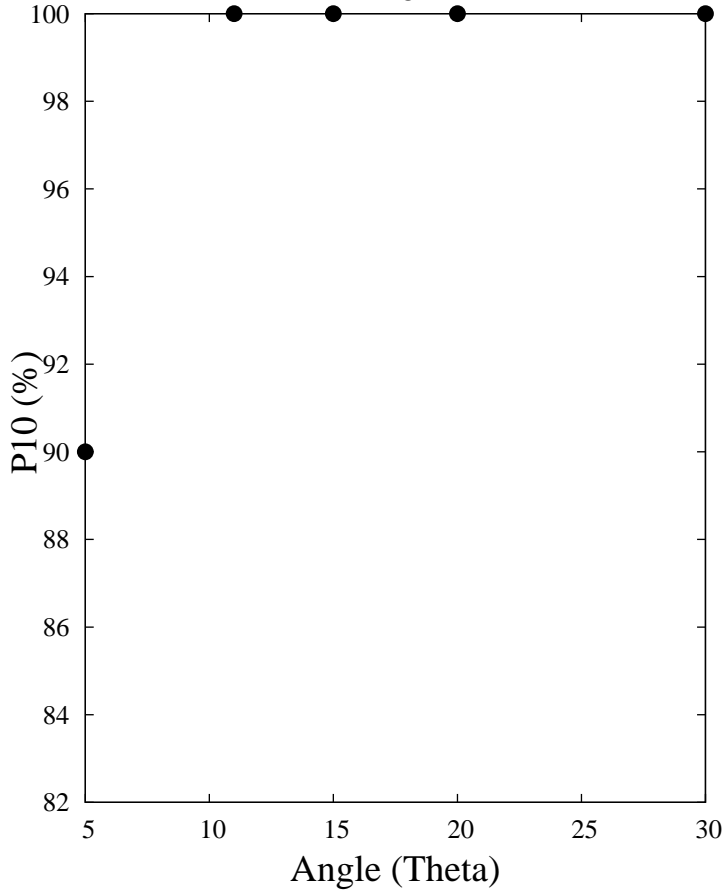
P10 factor - E_{high} (150+ MeV)
