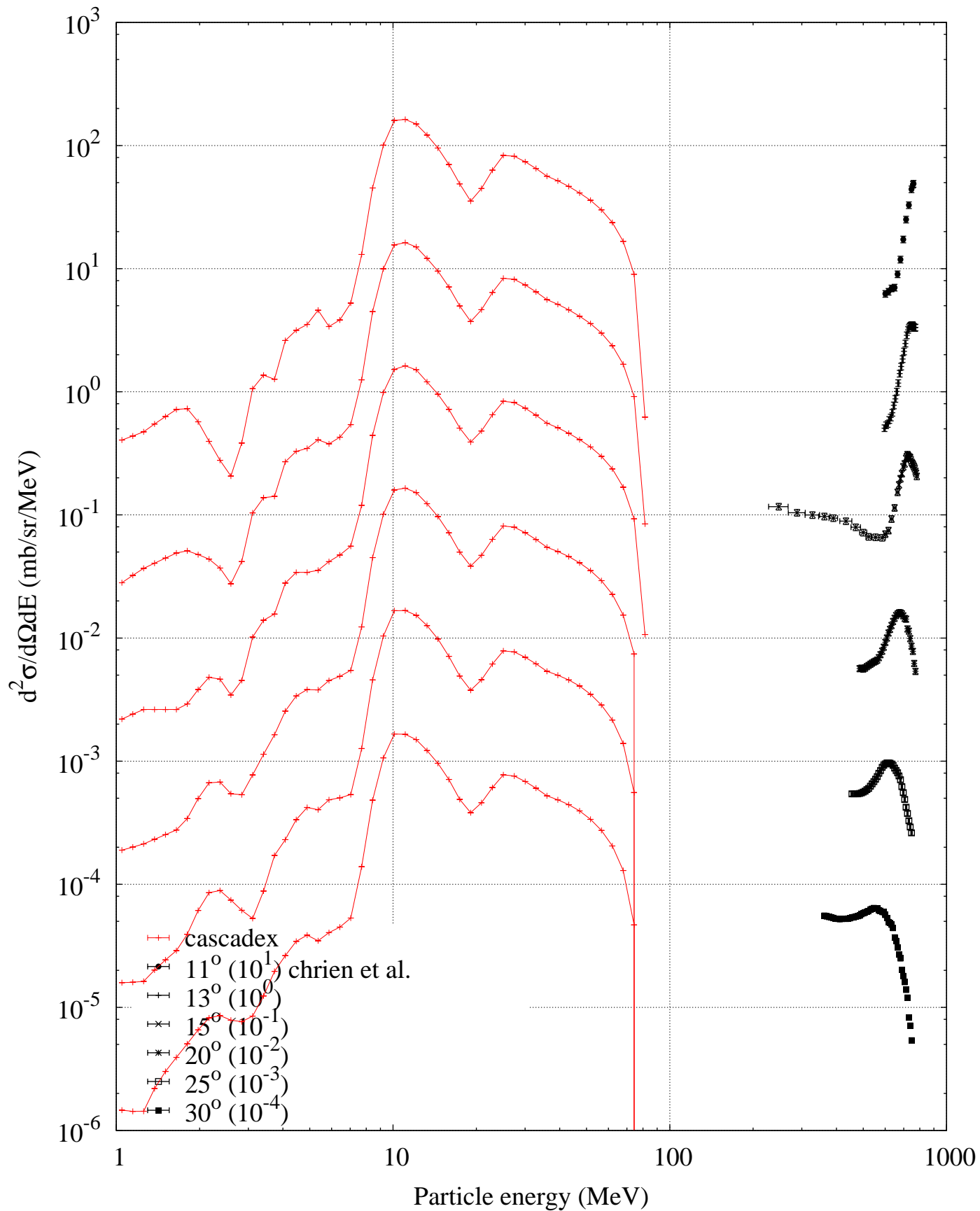
p (800 MeV) + Pb208 -- Particle spectrum
