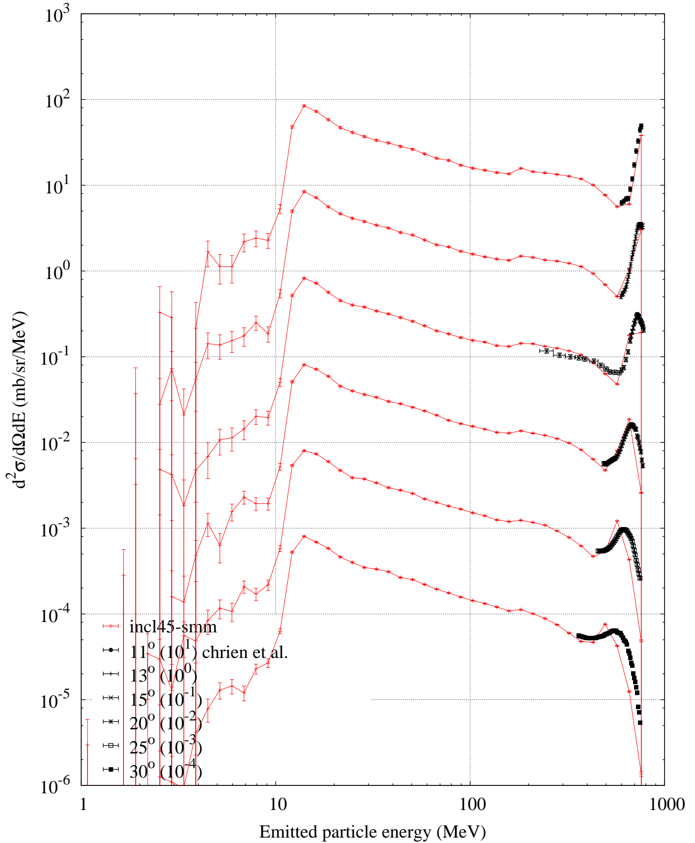
p (800 MeV) + Pb208 -- Proton spectrum
