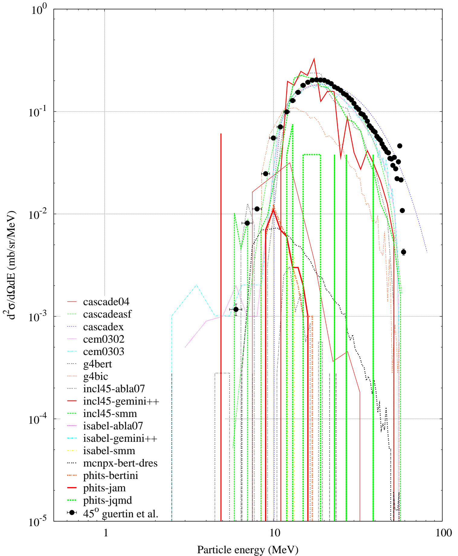
p (63 MeV) + Pb208 -- Triton spectrum
