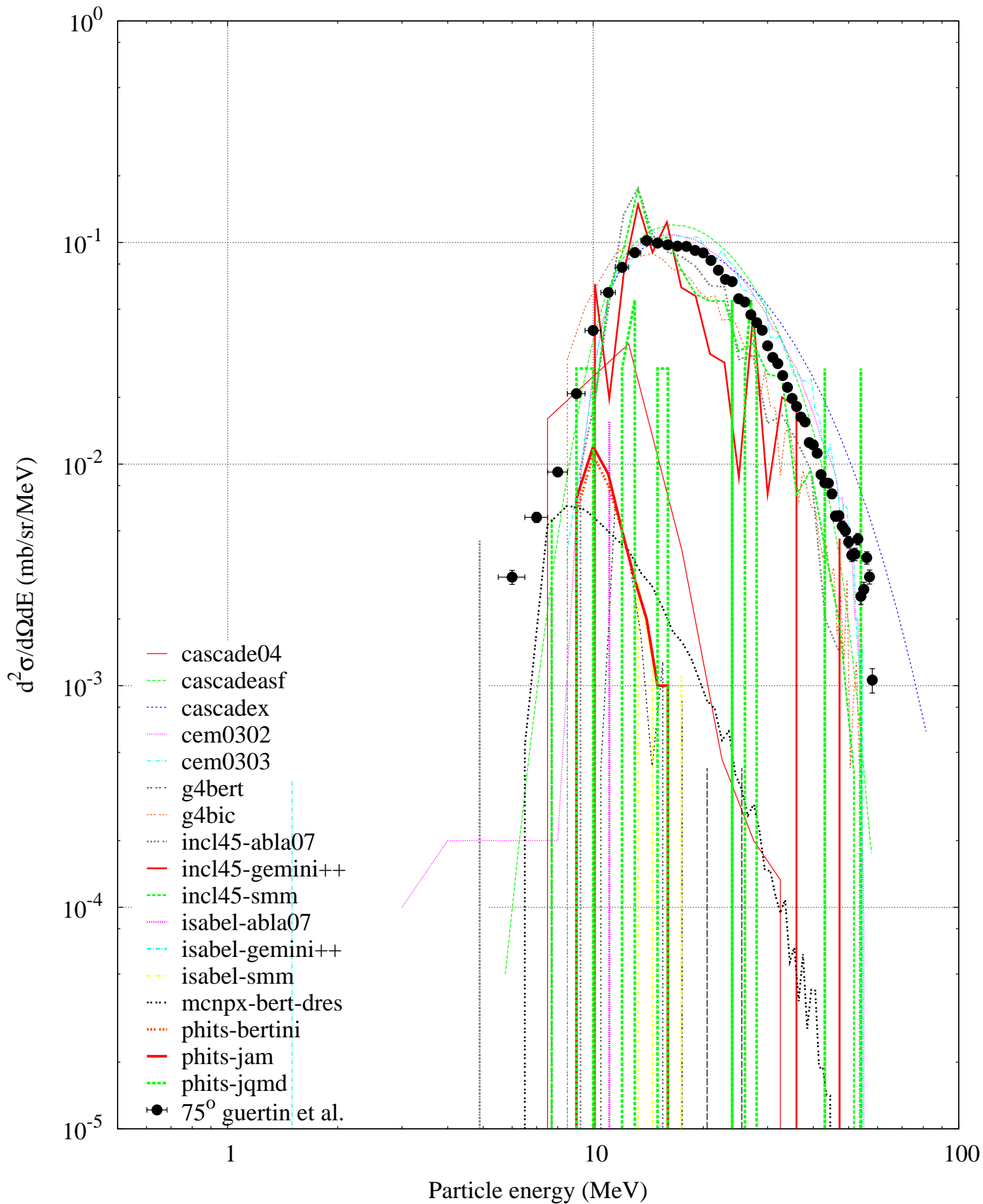
p (63 MeV) + Pb208 -- Triton spectrum
