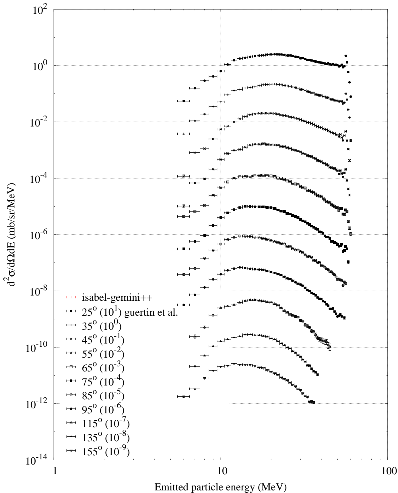
p (63 MeV) + Pb208 -- Tritium spectrum
