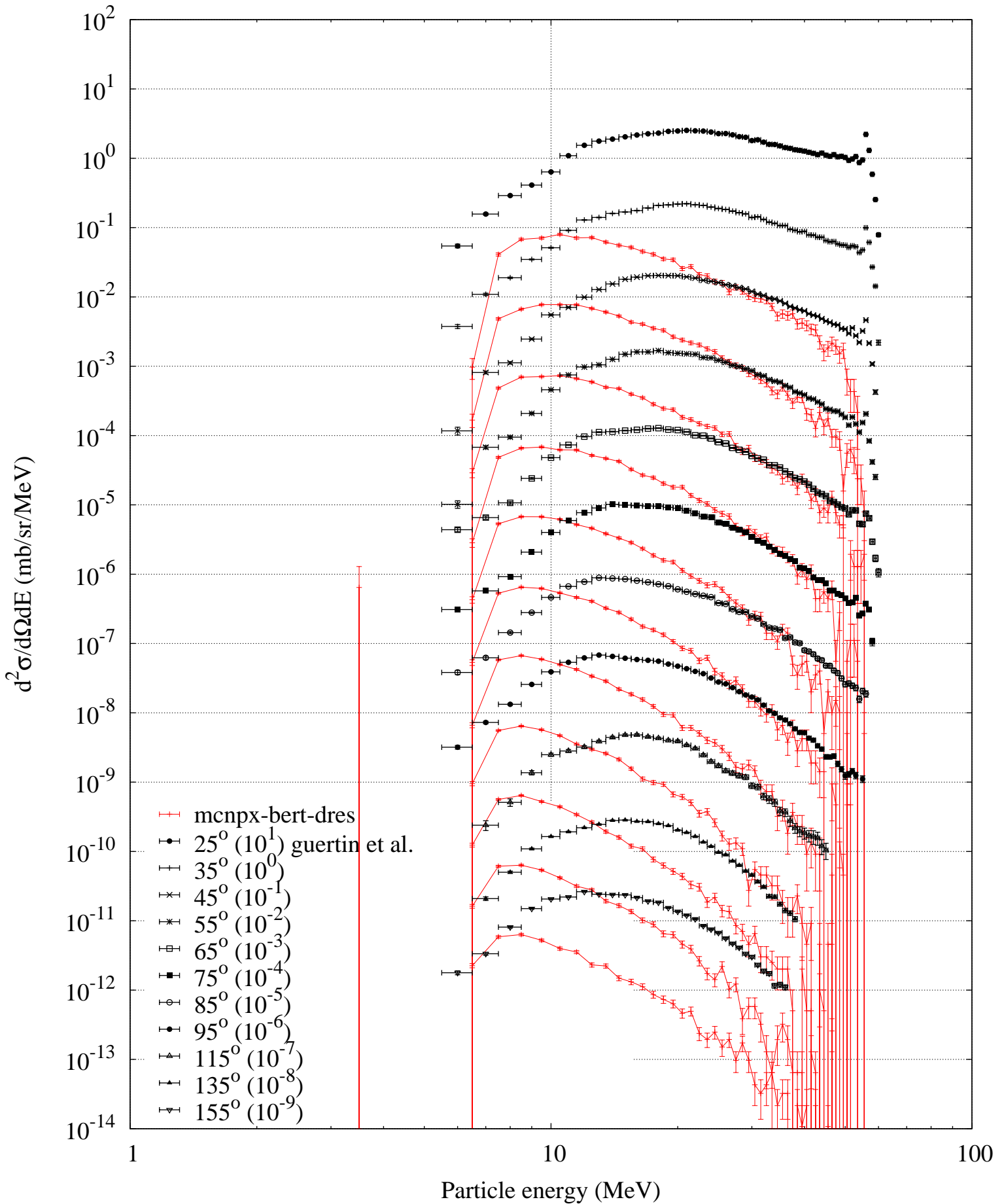
p (63 MeV) + Pb208 -- Triton spectrum
