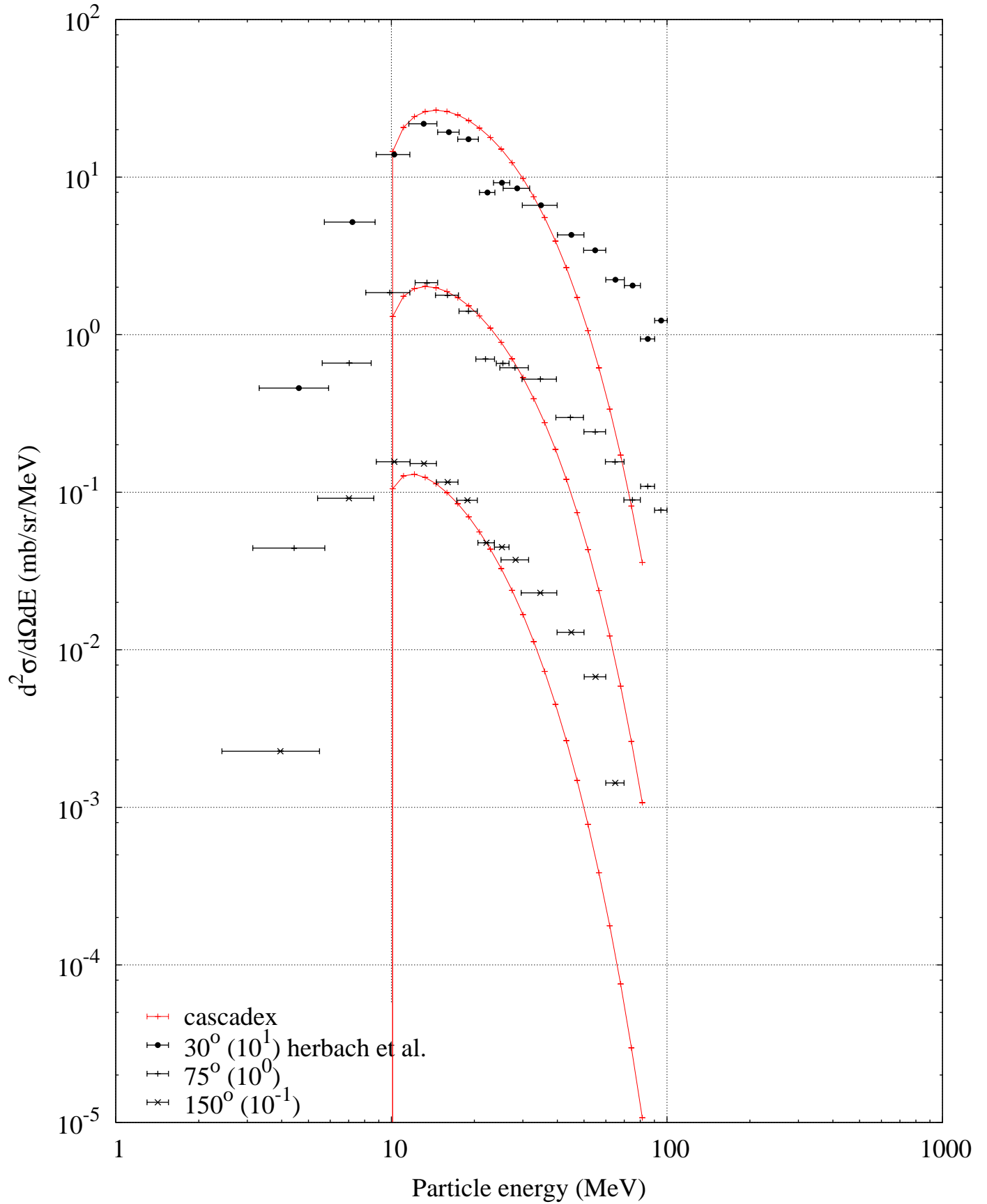
p (1200 MeV) + Ta -- Particle spectrum
