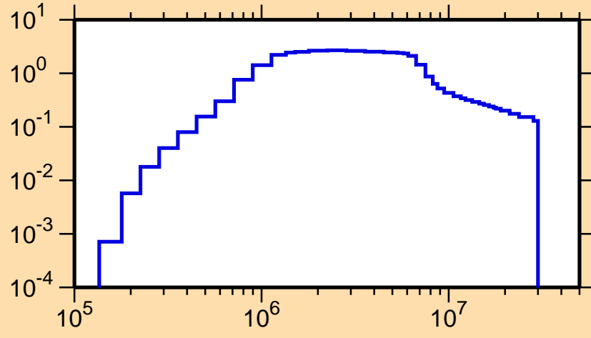
\sigma vs. E for ^{238}\text{U} (mt851)
