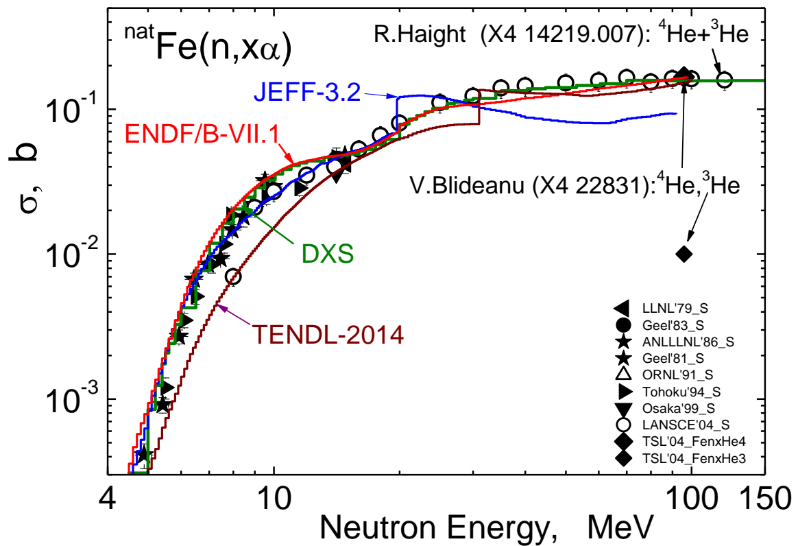
Fig. 1. He-4 production cross sections for natural Iron: experimental data and evaluations.
