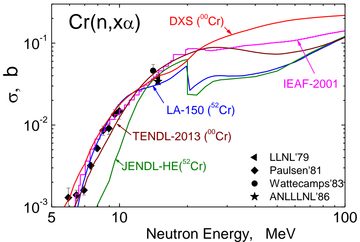
Fig. 2. He-4 production cross sections for natural Chromium: experimental data and evaluations.
