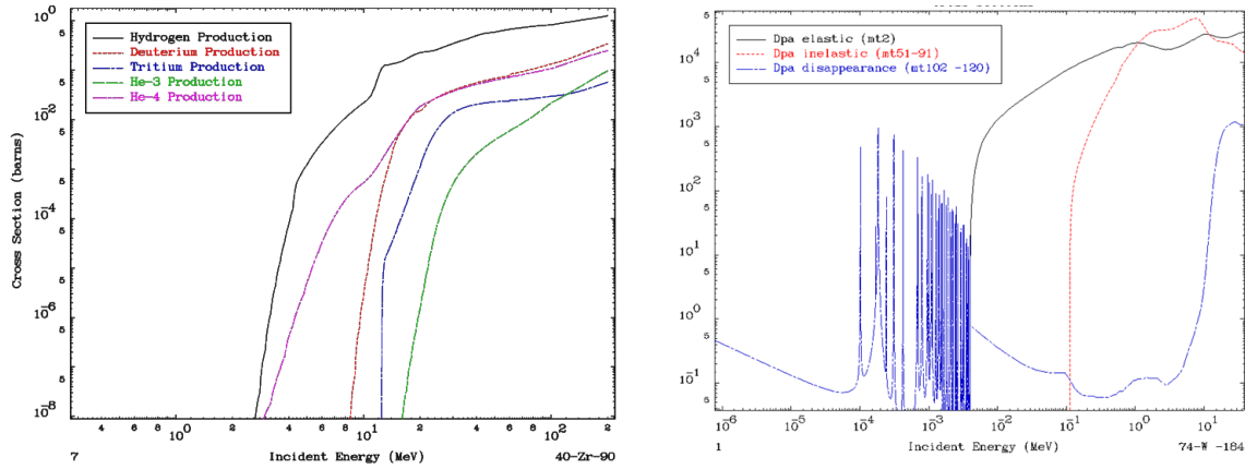
Figure 1. Gas production cross sections on ^{90}\text{Zr} , and partial displacement cross sections for ^{184}\text{W} .
