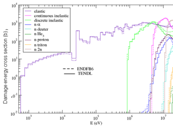
Fig. 2a. Calculation of the damage energy cross section versus the neutron energy on ^{56}\text{Fe} atoms with the DART code using both ENDFB-VI (dashed line) and TENDL-2012 (full line).
