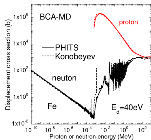
Fig. 2. Comparison between the \sigma_{BCA-MD} that was calculated using the PHITS and the data that was taken from the KIT data file.
