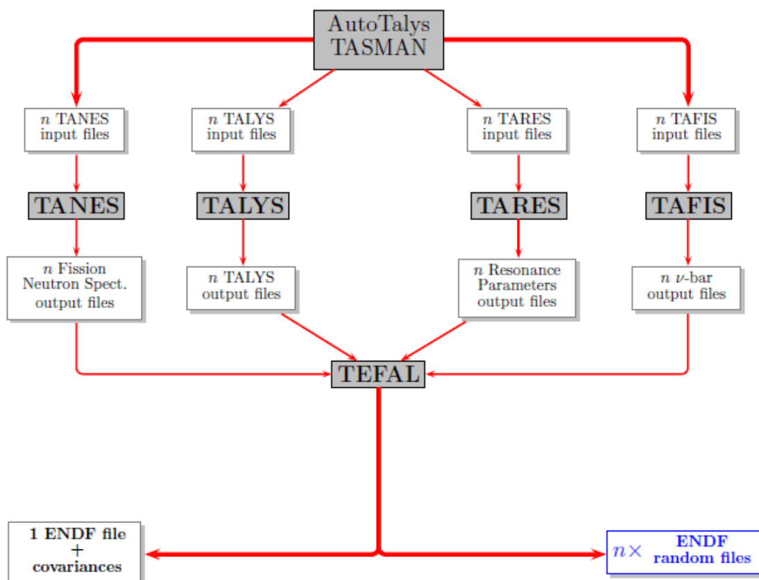
Figure 1. Flowchart of the nuclear data file evaluation and production process with the TALYS system.
