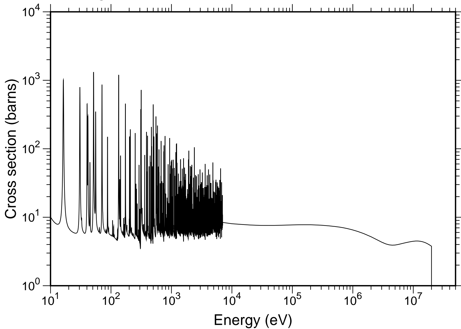
Natural Ag Total Cross-section - JENDL-4.0
