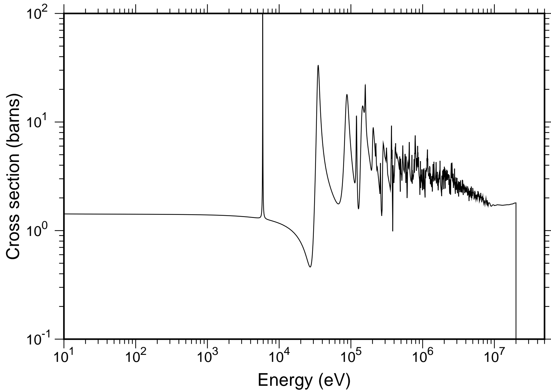
Natural Al Total Cross-section - JENDL-4.0
