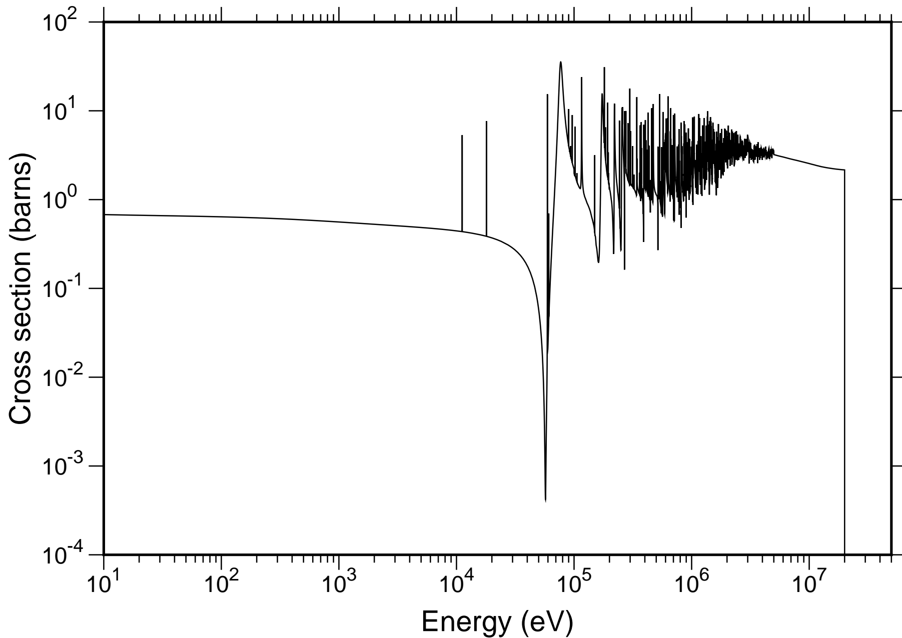
Natural Ar Total Cross-section - JENDL-4.0
