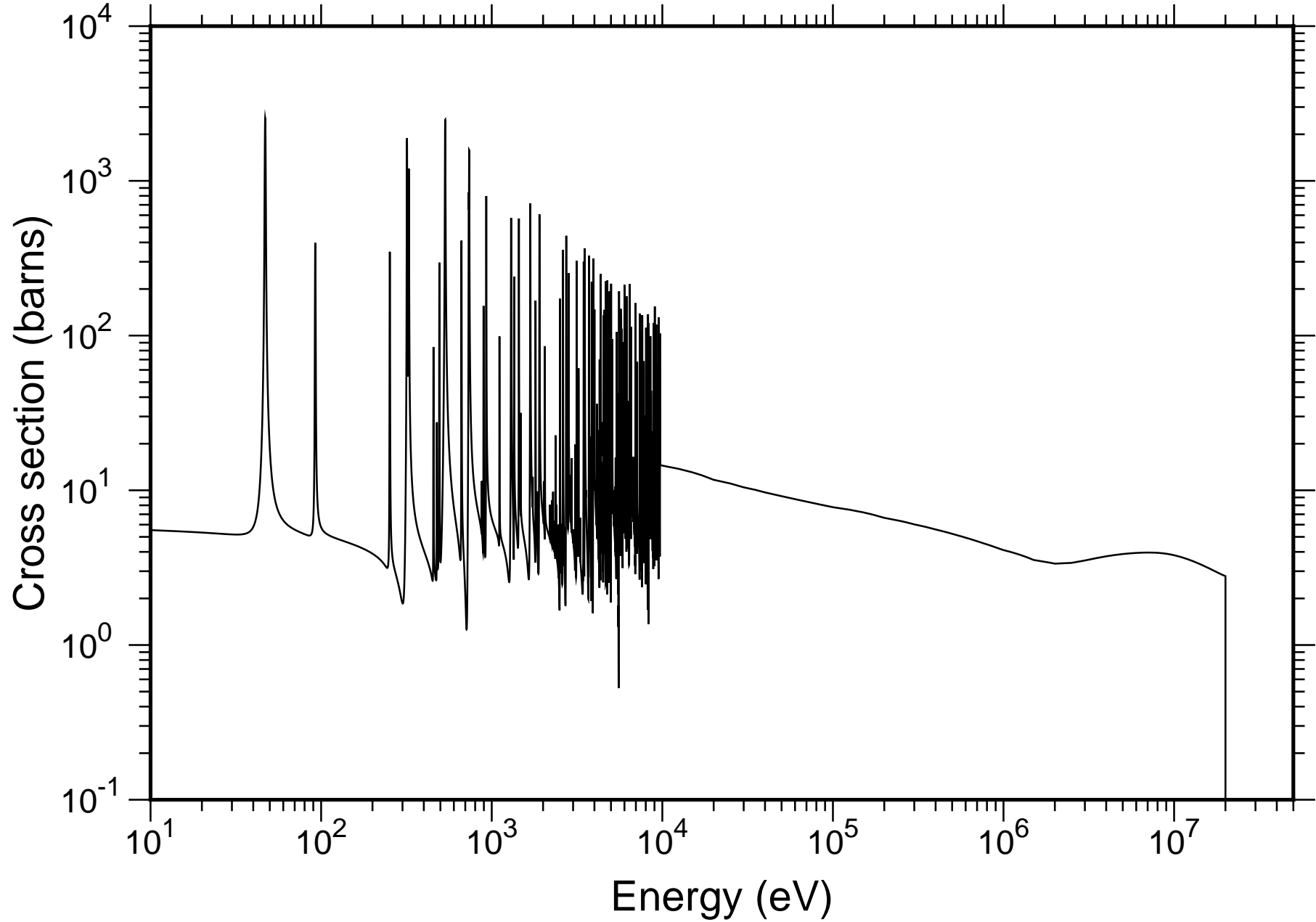
Natural As Total Cross-section - JENDL-4.0
