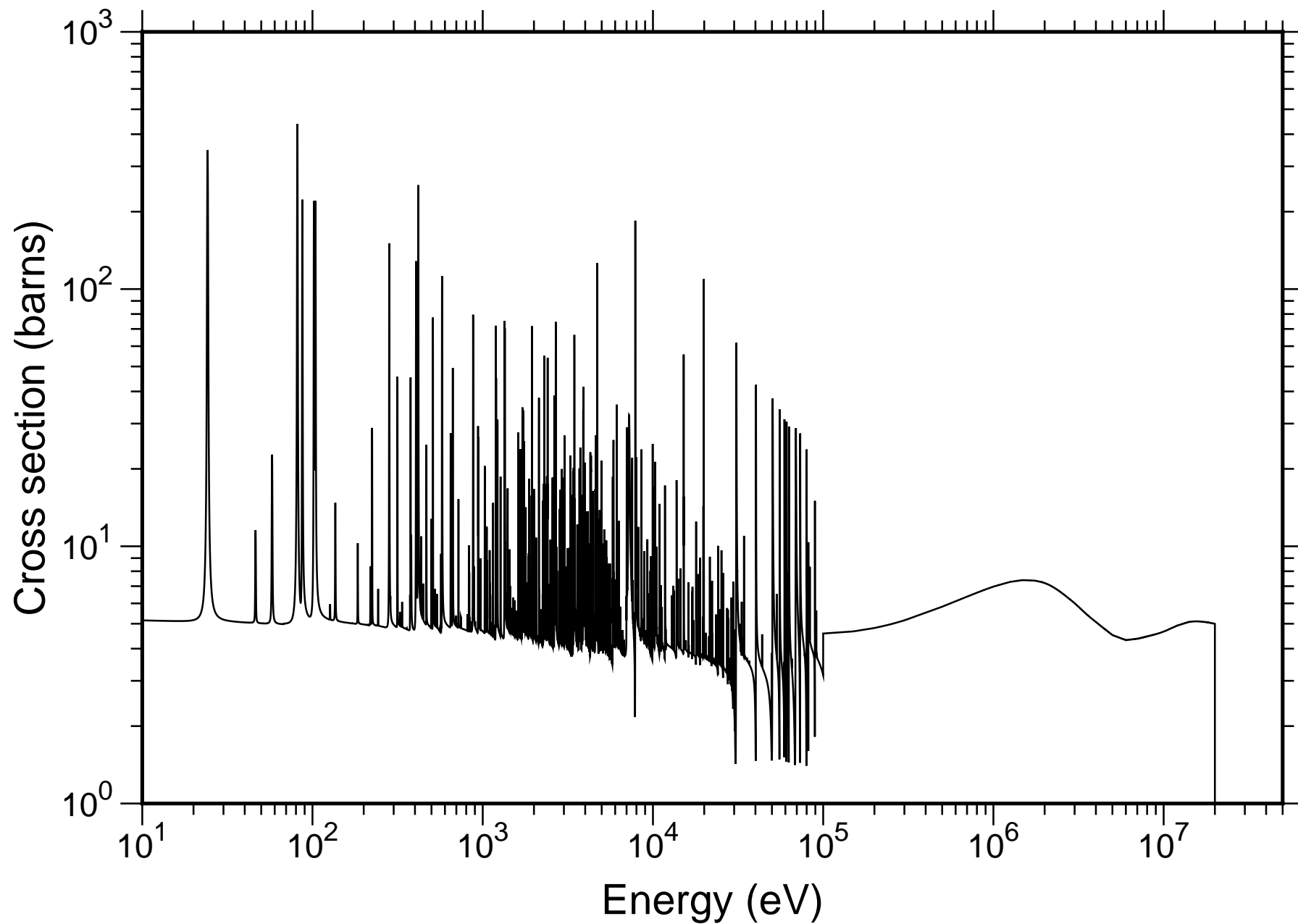
Natural Ba Total Cross-section - JENDL-4.0
