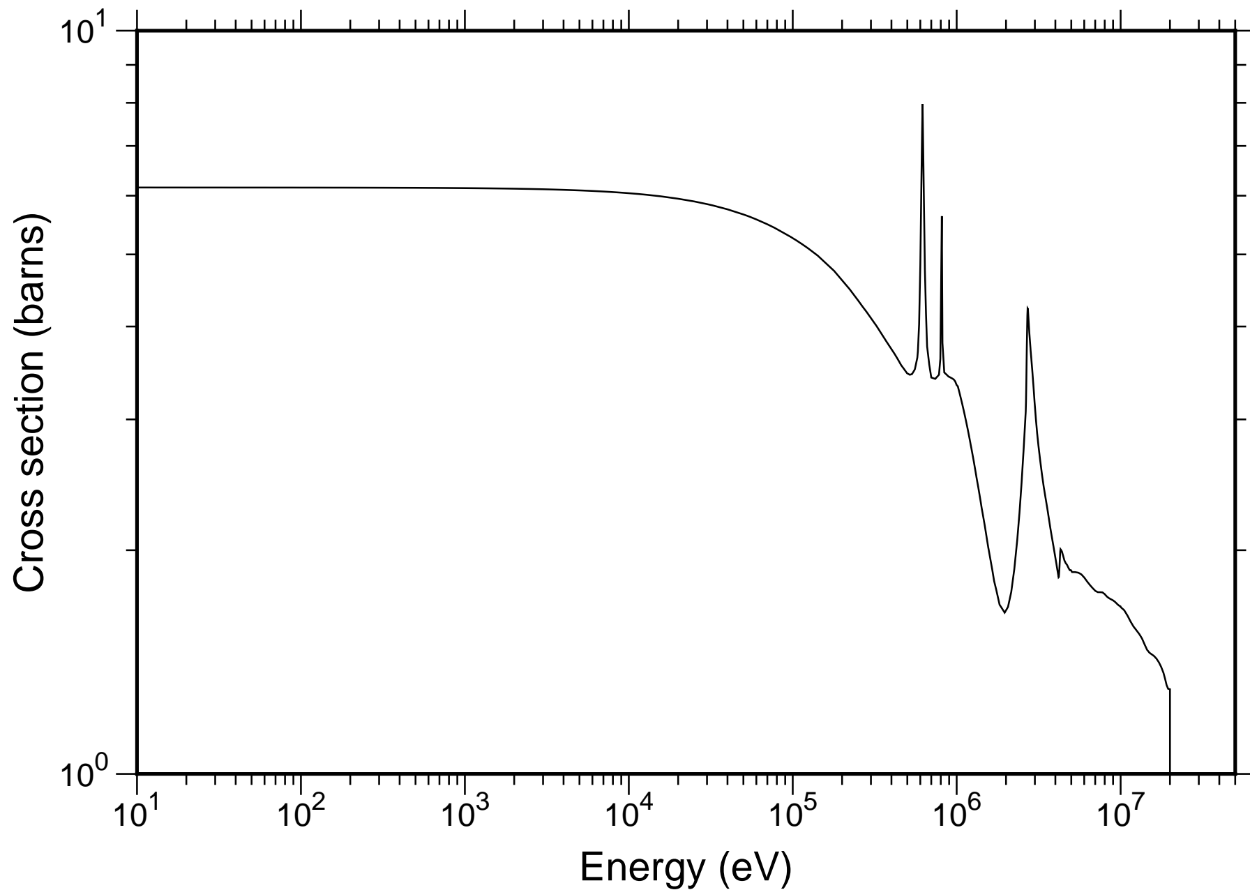
Natural Be Total Cross-section - JENDL-4.0
