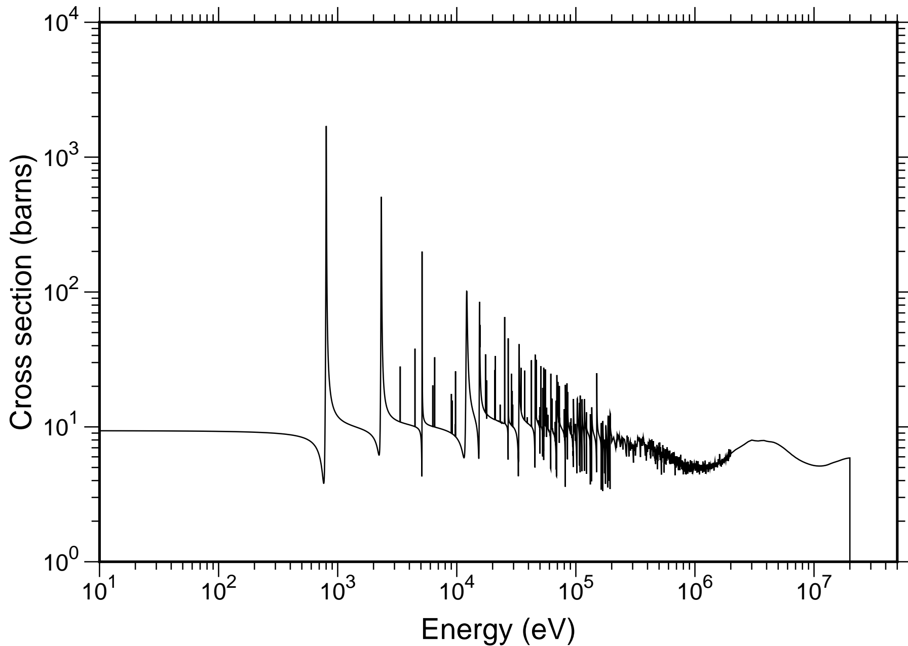
Natural Bi Total Cross-section - JENDL-4.0
