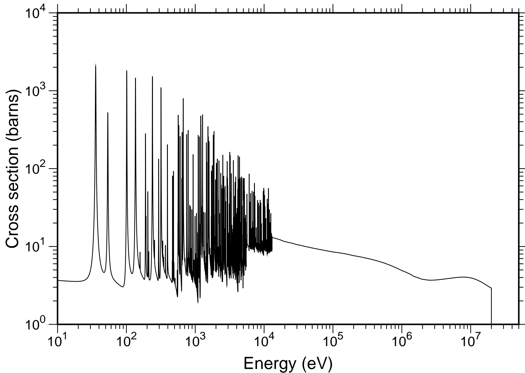
Natural Br Total Cross-section - JENDL-4.0
