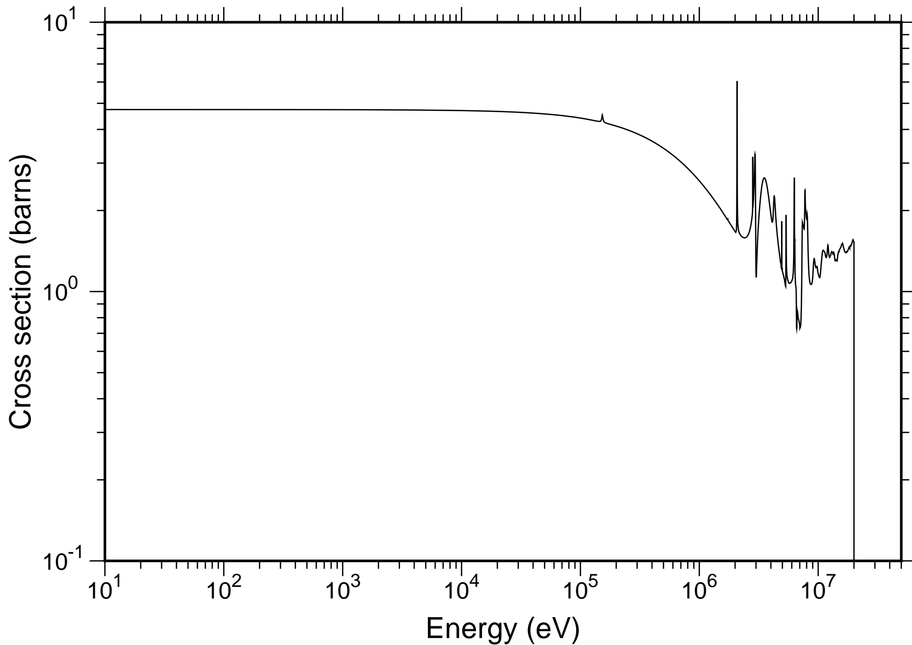
Natural C Total Cross-section - JENDL-4.0
