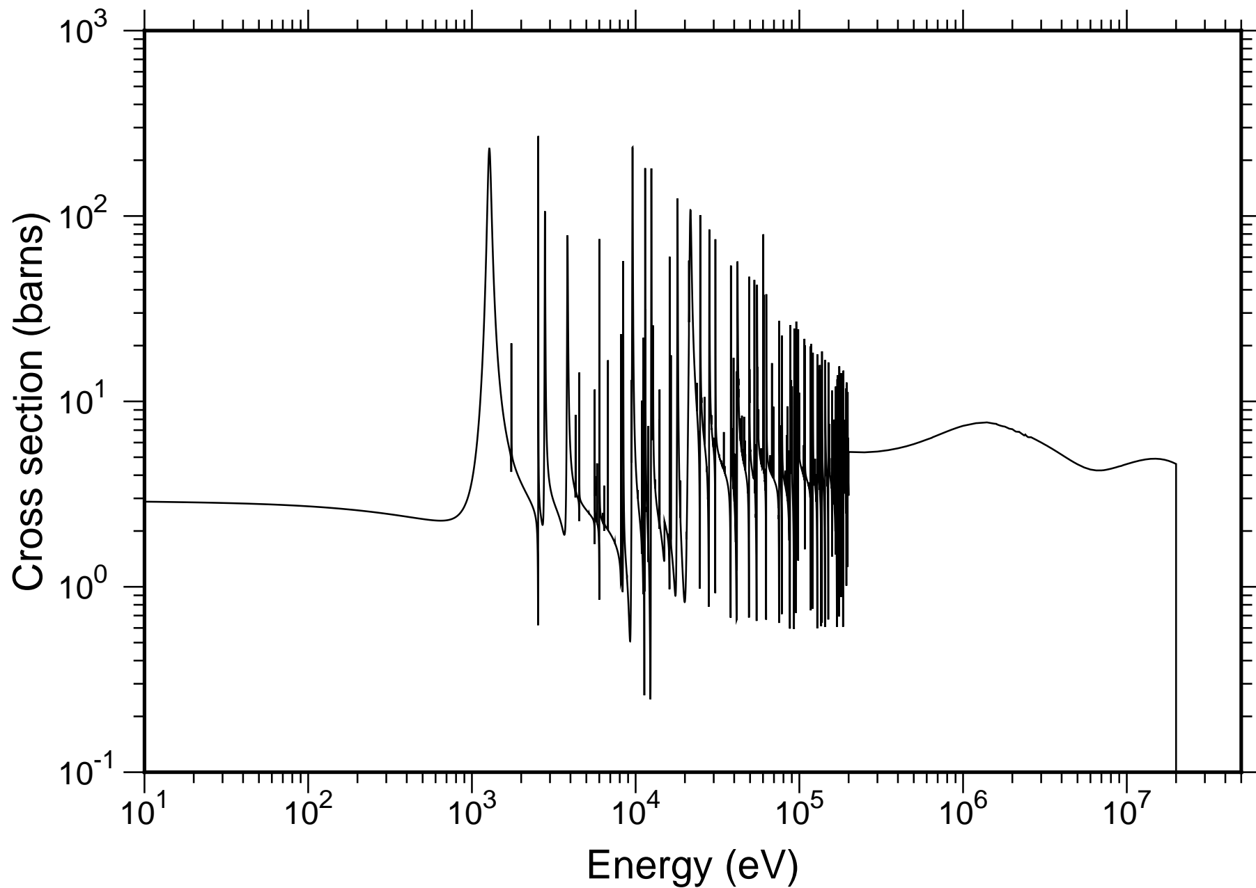
Natural Ce Total Cross-section - JENDL-4.0
