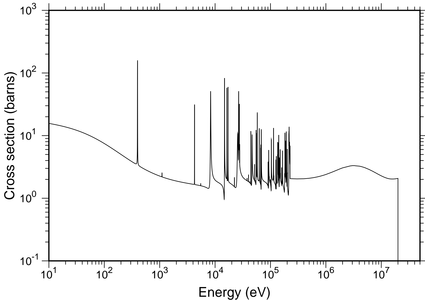
Natural Cl Total Cross-section - JENDL-4.0
