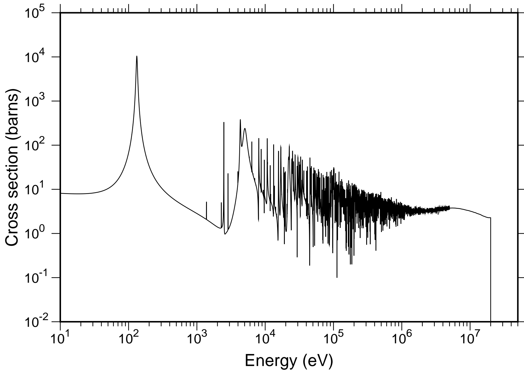
Natural Co Total Cross-section - JENDL-4.0
