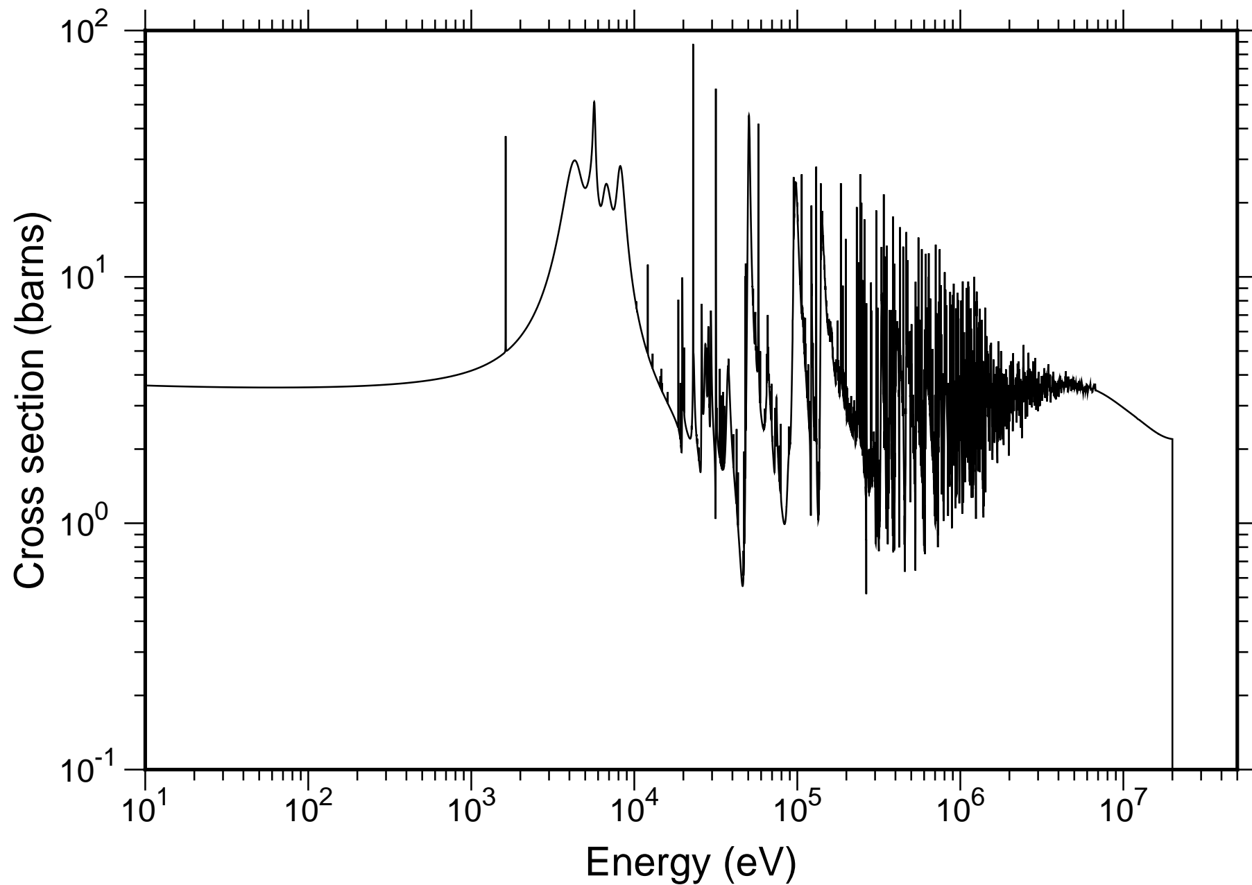
Natural Cr Total Cross-section - JENDL-4.0
