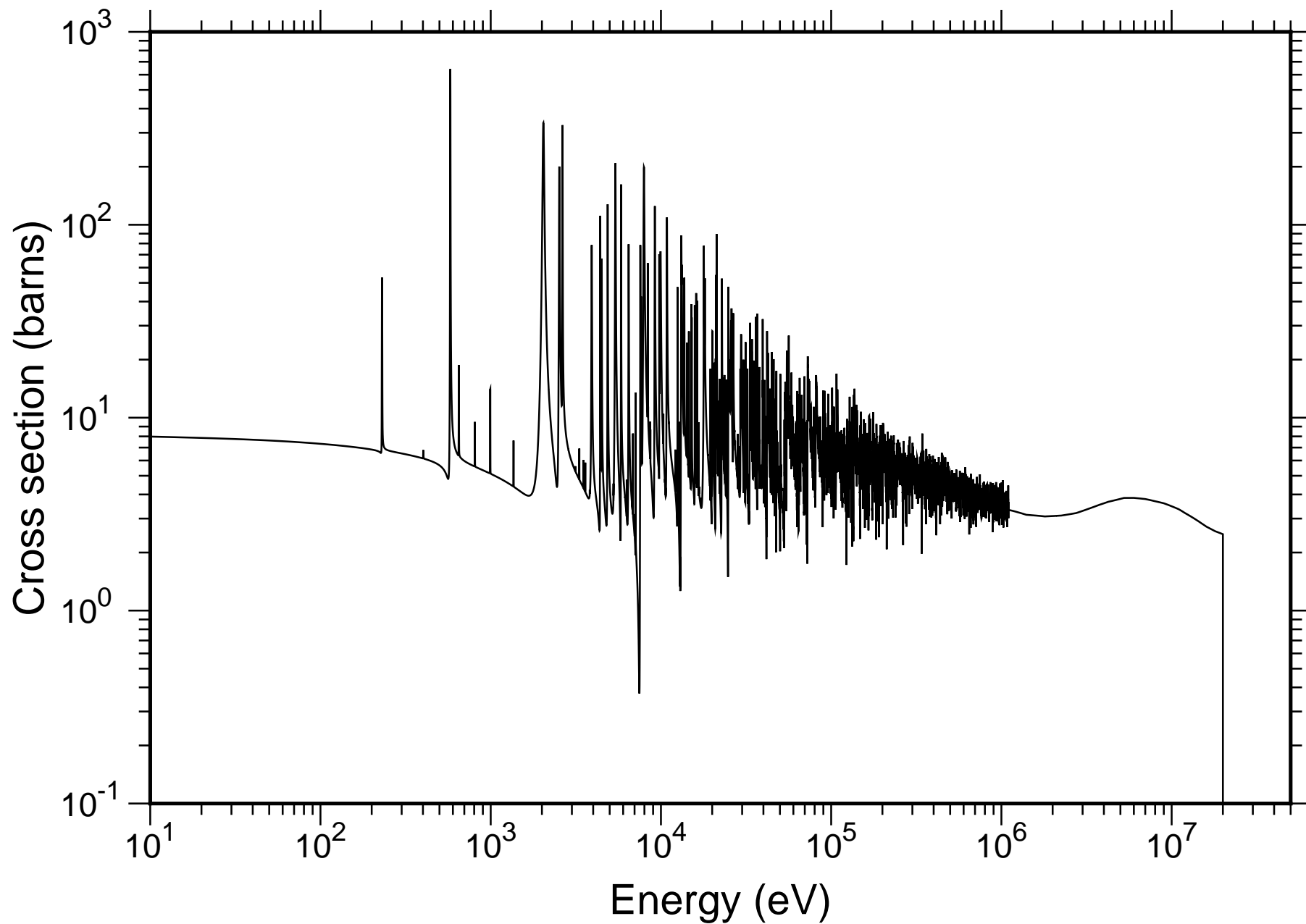
Natural Cu Total Cross-section - JENDL-4.0
