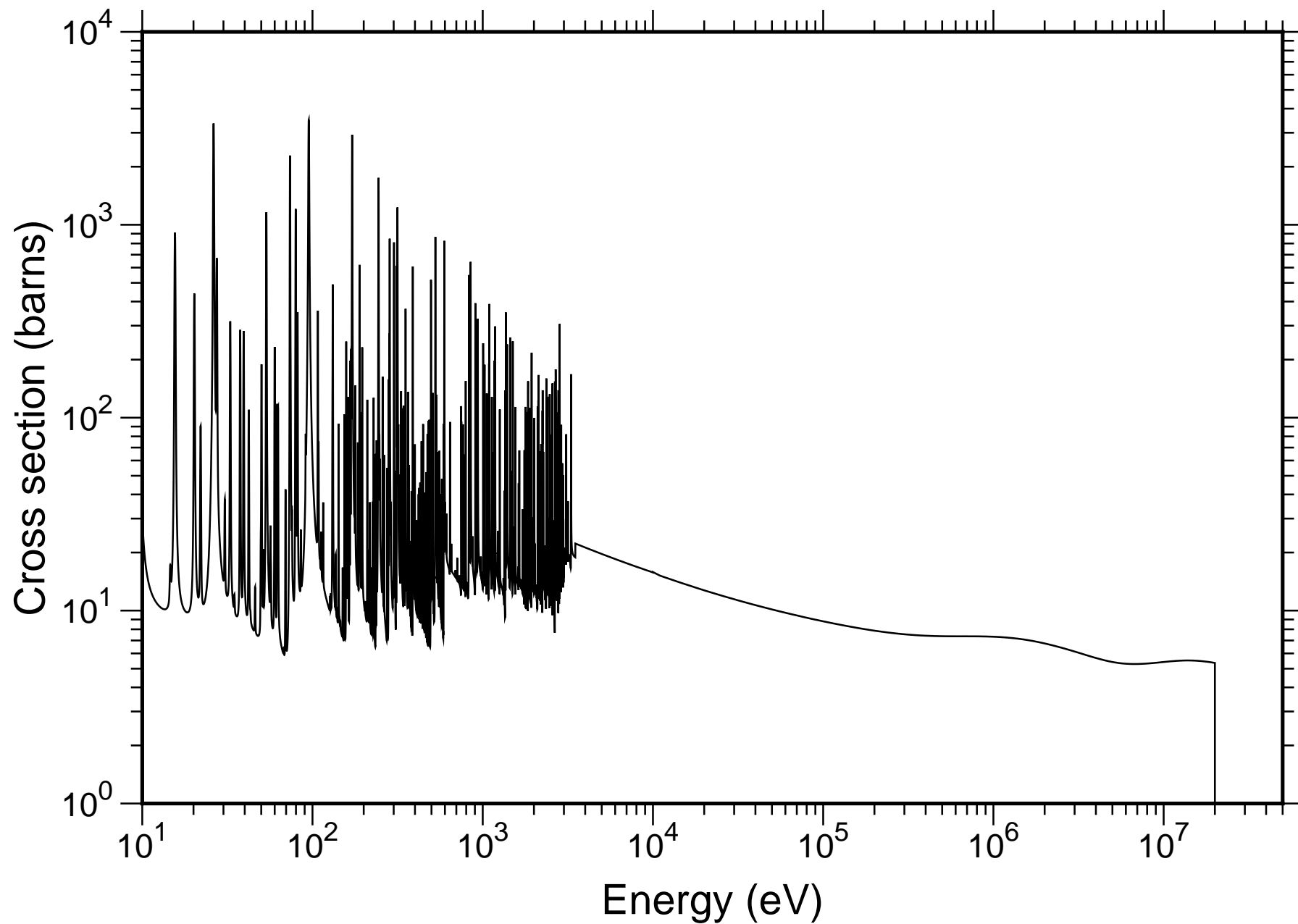
Natural Er Total Cross-section - JENDL-4.0
