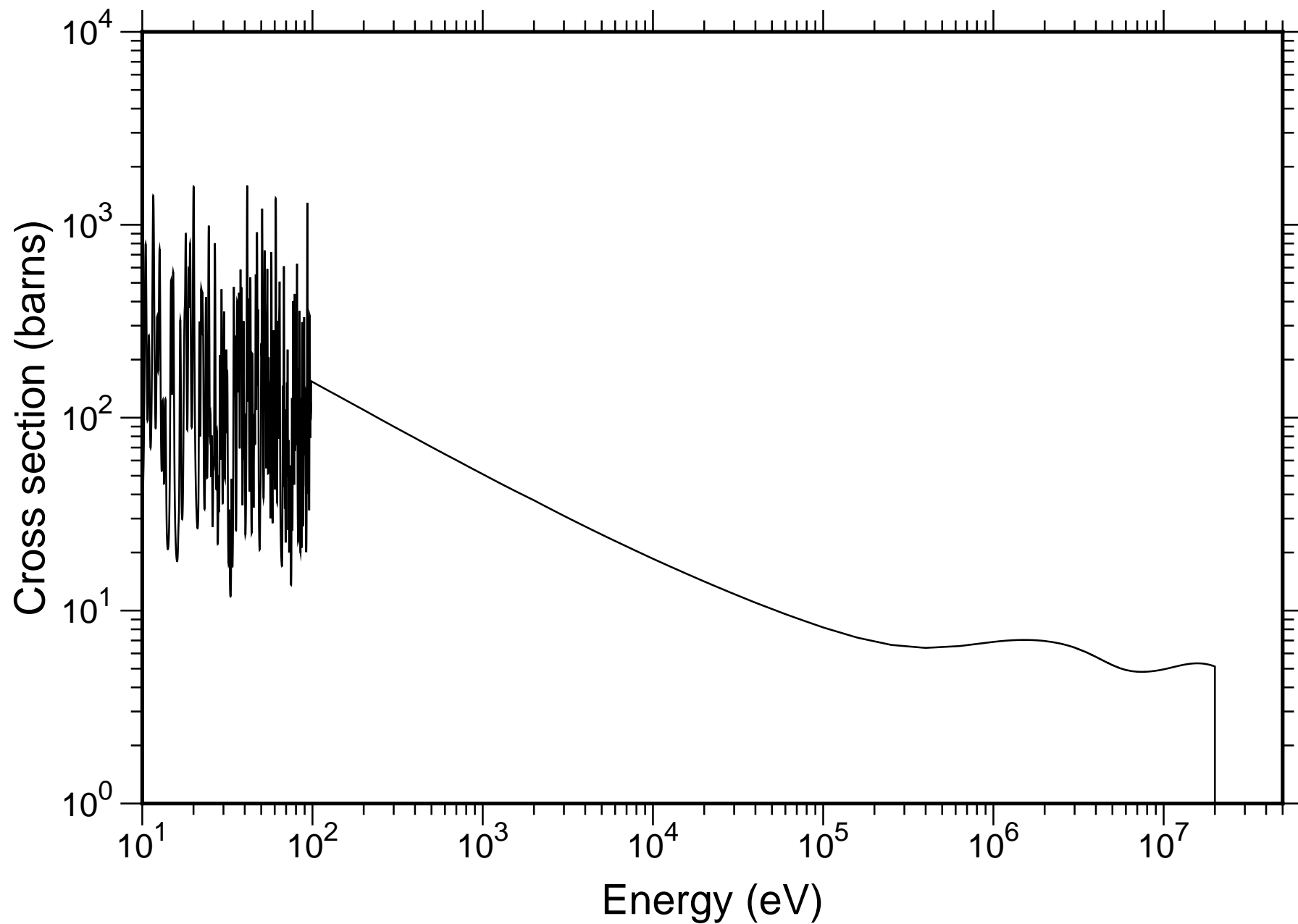
Natural Eu Total Cross-section - JENDL-4.0
