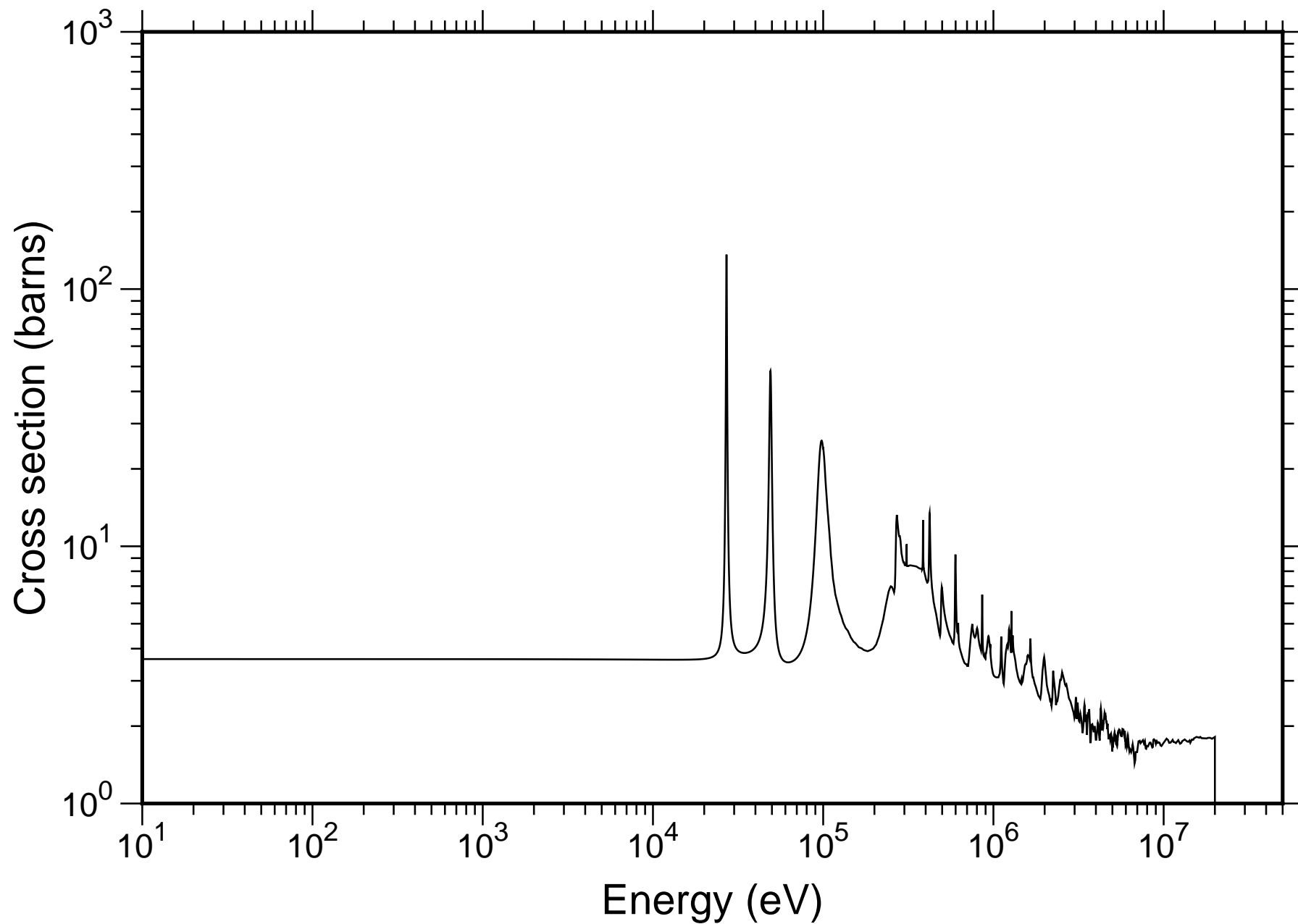
Natural F Total Cross-section - JENDL-4.0
