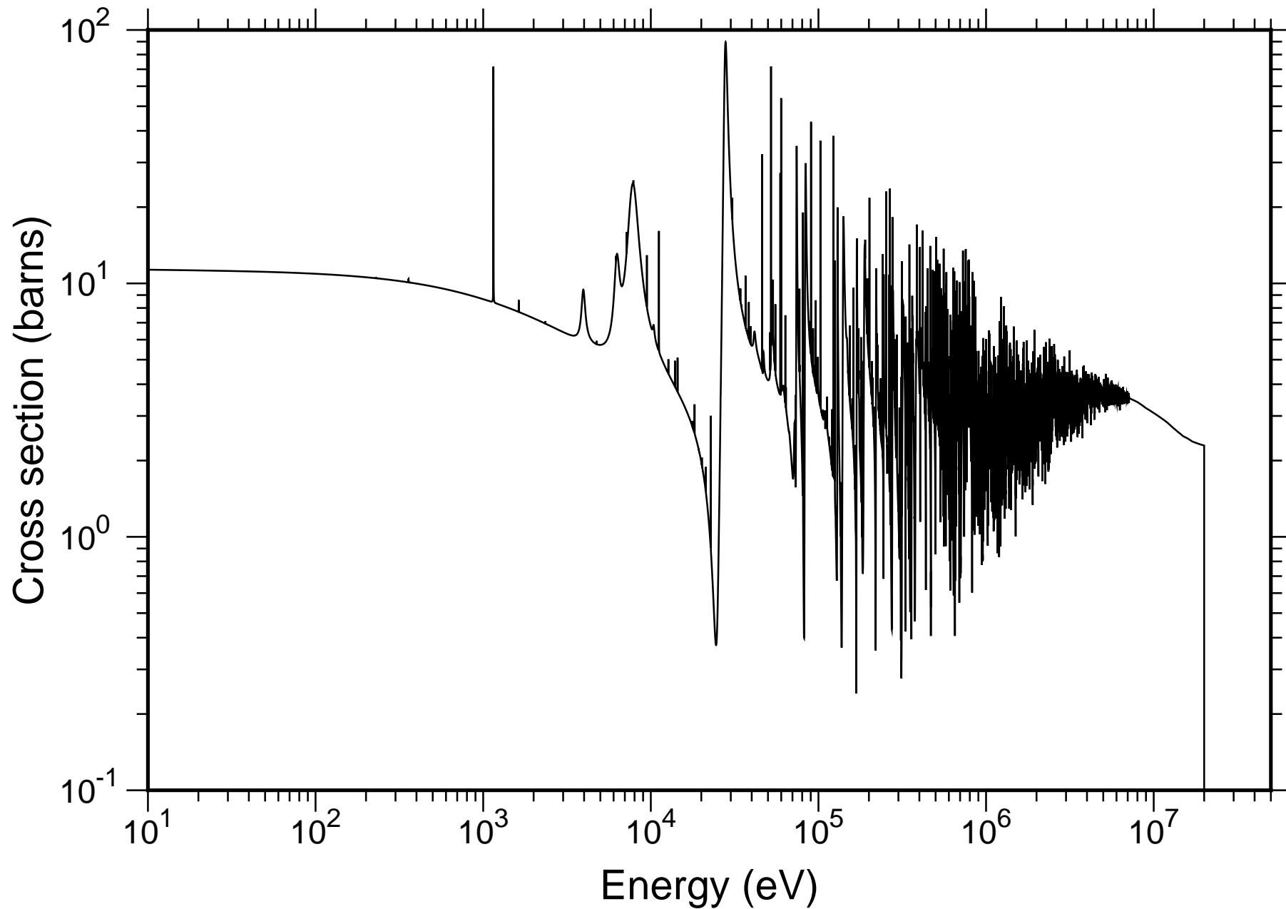
Natural Fe Total Cross-section - JENDL-4.0
