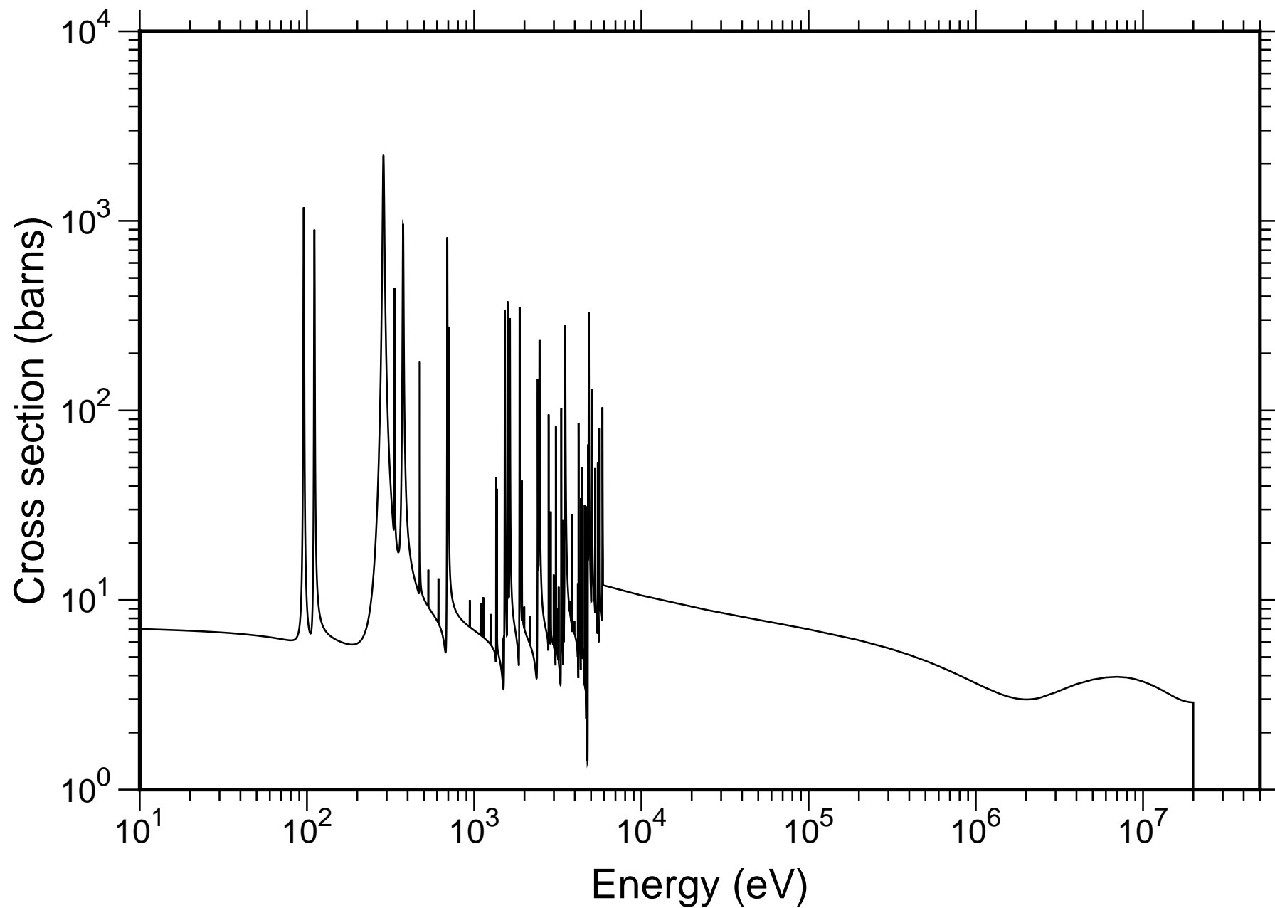
Natural Ga Total Cross-section - JENDL-4.0
