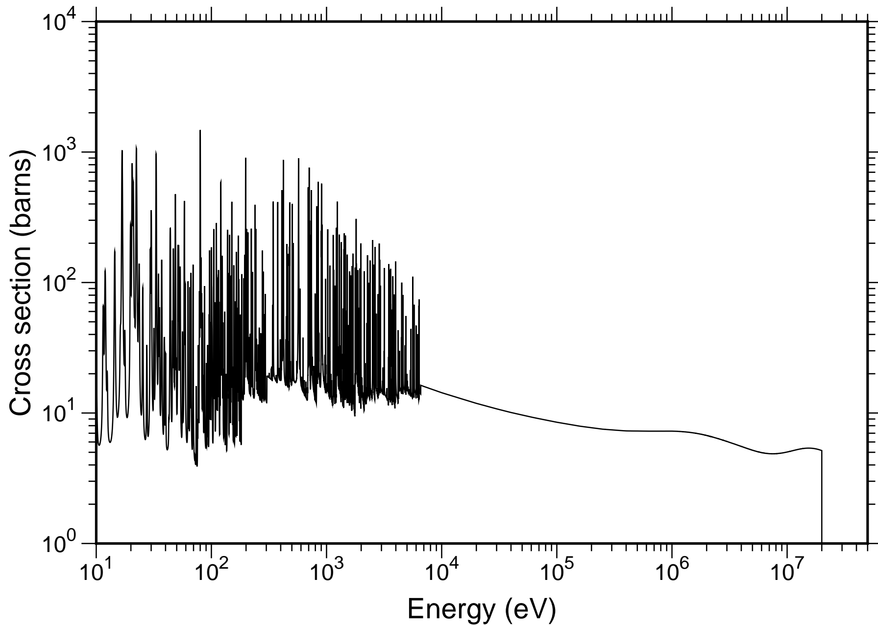
Natural Gd Total Cross-section - JENDL-4.0
